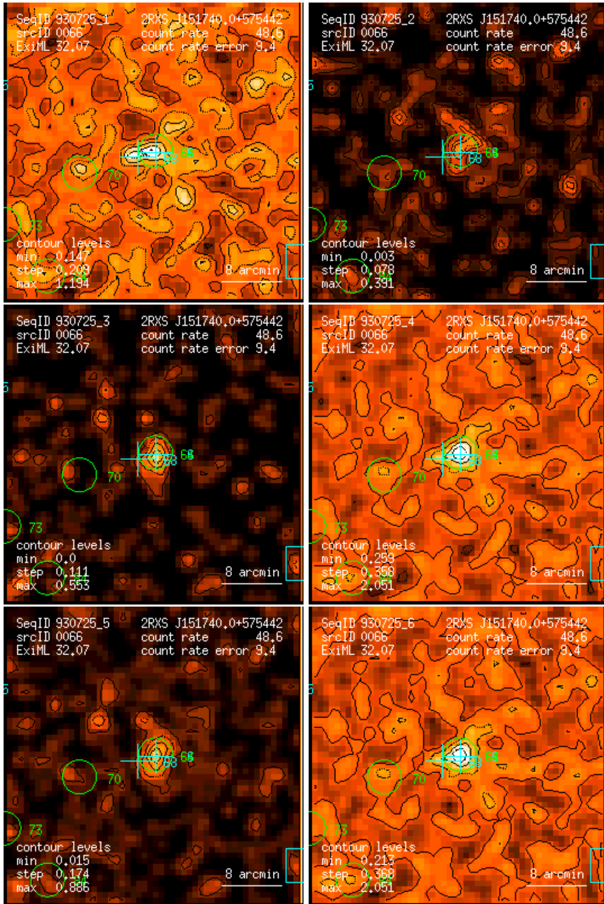
Figure 66: RASS 930725: detection 0066: band rate images, Gaussian filter: (1) PSPC channels 11 – 41, (2) 52 – 90, (3) 91 – 201, (4) 11 – 235, (5) 52 – 201, (6) 11 – 201. Broad band rates in counts/ks. Band rate contour levels in counts/ks/arcmin 2 .
