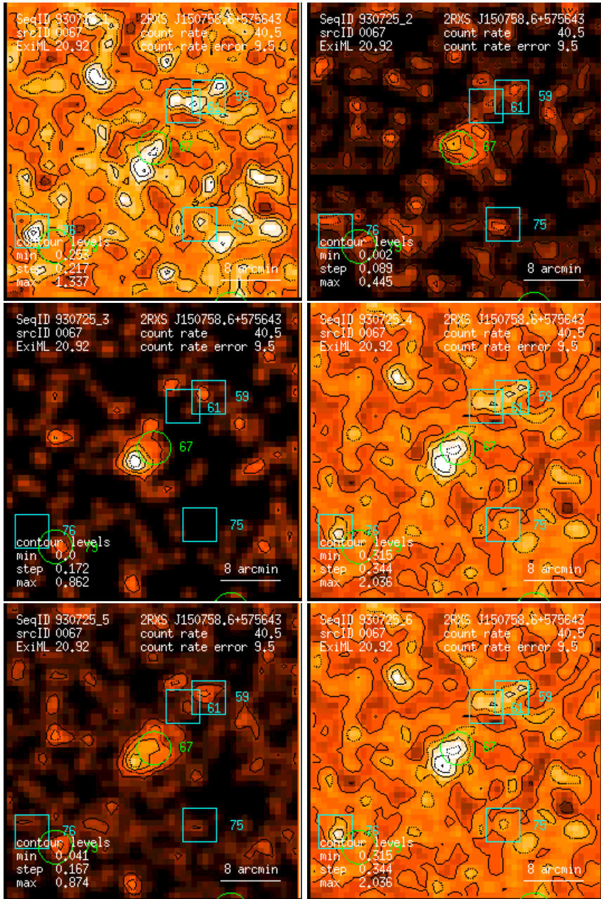
Figure 67: RASS 930725: detection 0067: band rate images, Gaussian filter: (1) PSPC channels 11 – 41, (2) 52 – 90, (3) 91 – 201, (4) 11 – 235, (5) 52 – 201, (6) 11 – 201. Broad band rates in counts/ks. Band rate contour levels in counts/ks/arcmin 2 .
