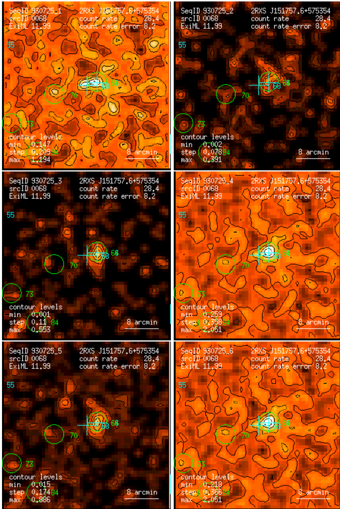
Figure 68: RASS 930725: detection 0068: band rate images, Gaussian filter: (1) PSPC channels 11 – 41, (2) 52 – 90, (3) 91 – 201, (4) 11 – 235, (5) 52 – 201, (6) 11 – 201. Broad band rates in counts/ks. Band rate contour levels in counts/ks/arcmin 2 .
