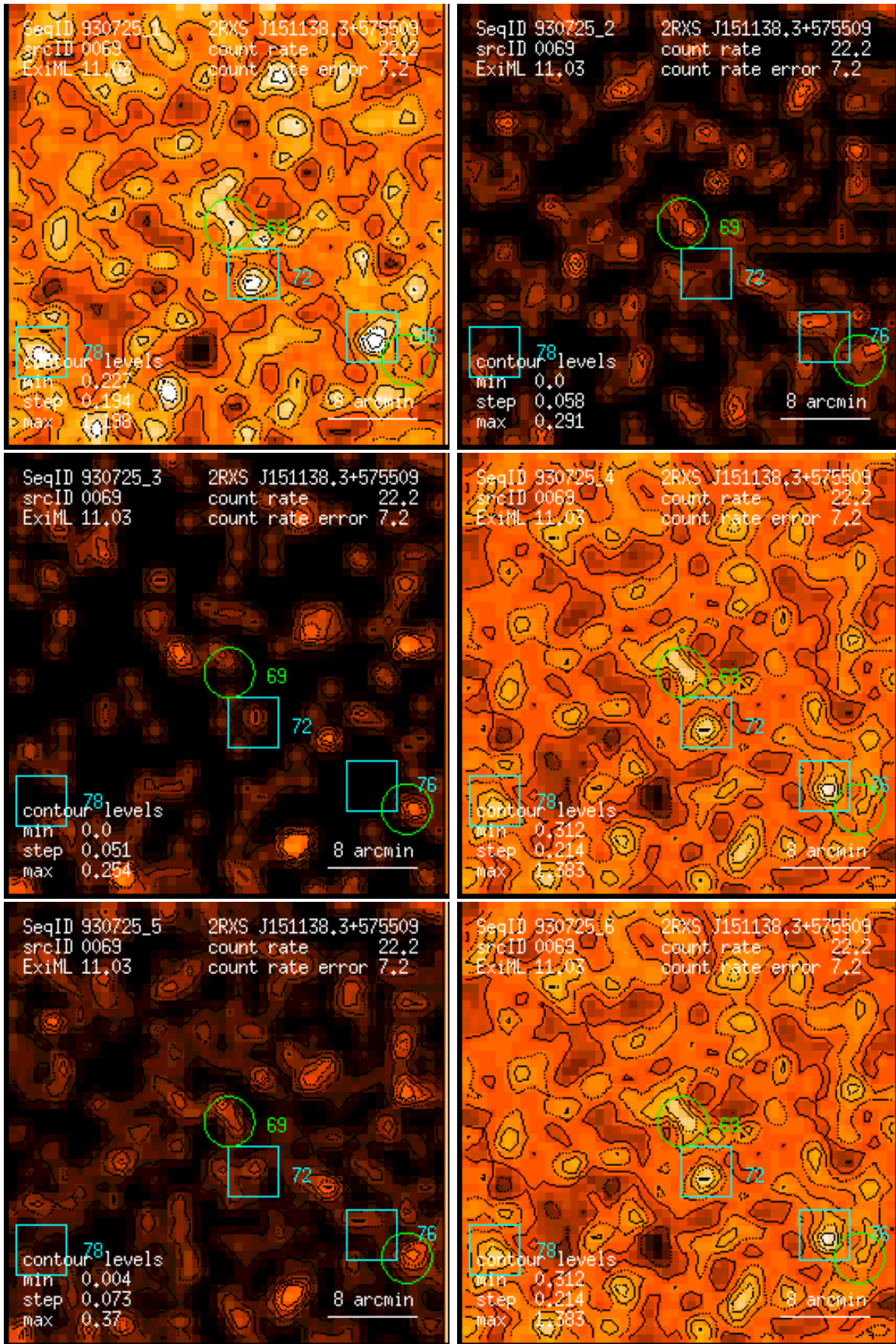
Figure 69: RASS 930725: detection 0069: band rate images, Gaussian filter: (1) PSPC channels 11 – 41, (2) 52 – 90, (3) 91 – 201, (4) 11 – 235, (5) 52 – 201, (6) 11 – 201. Broad band rates in counts/ks. Band rate contour levels in counts/ks/arcmin 2 .
