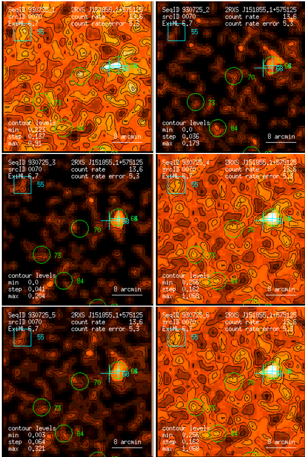
Figure 70: RASS 930725: detection 0070: band rate images, Gaussian filter: (1) PSPC channels 11 – 41, (2) 52 – 90, (3) 91 – 201, (4) 11 – 235, (5) 52 – 201, (6) 11 – 201. Broad band rates in counts/ks. Band rate contour levels in counts/ks/arcmin 2 .
