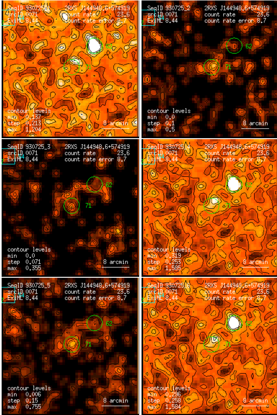
Figure 71: RASS 930725: detection 0071: band rate images, Gaussian filter: (1) PSPC channels 11 – 41, (2) 52 – 90, (3) 91 – 201, (4) 11 – 235, (5) 52 – 201, (6) 11 – 201. Broad band rates in counts/ks. Band rate contour levels in counts/ks/arcmin 2 .
