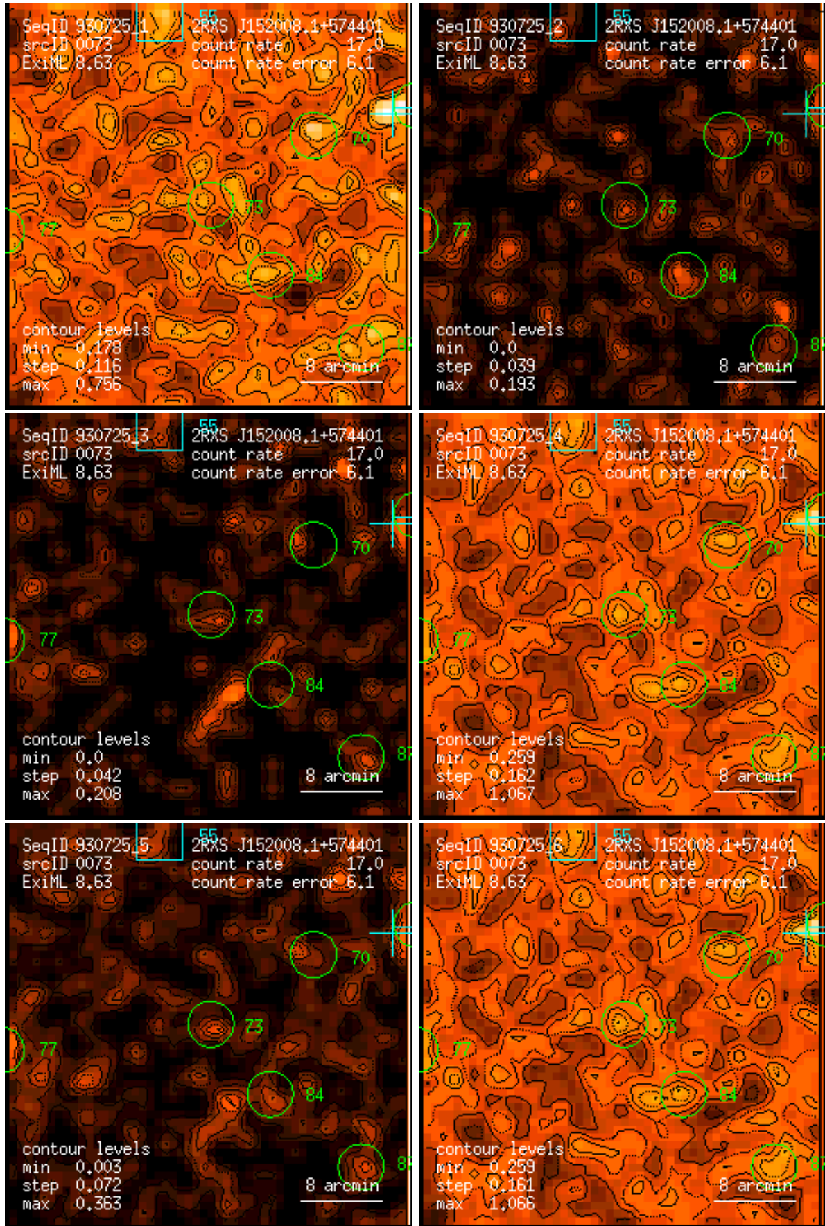
Figure 73: RASS 930725: detection 0073: band rate images, Gaussian filter: (1) PSPC channels 11 – 41, (2) 52 – 90, (3) 91 – 201, (4) 11 – 235, (5) 52 – 201, (6) 11 – 201. Broad band rates in counts/ks. Band rate contour levels in counts/ks/arcmin 2 .
