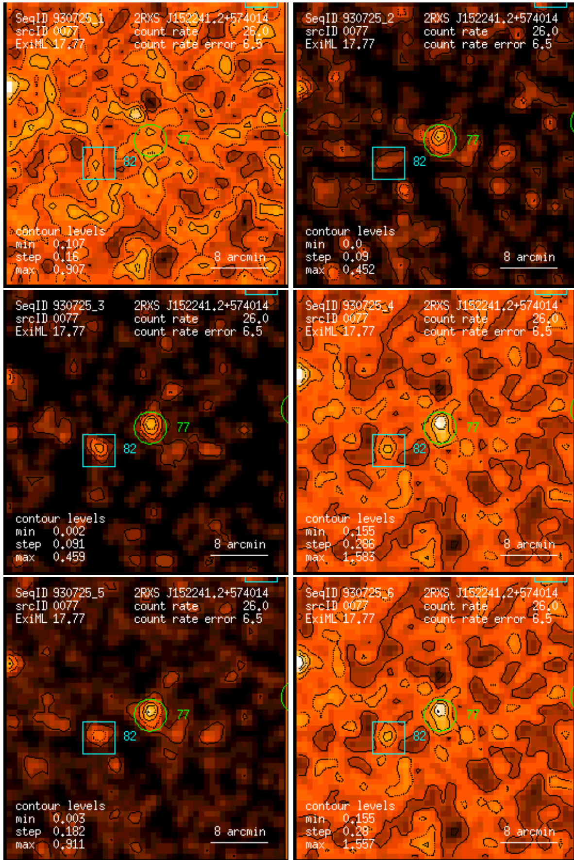
Figure 77: RASS 930725: detection 0077: band rate images, Gaussian filter: (1) PSPC channels 11 – 41, (2) 52 – 90, (3) 91 – 201, (4) 11 – 235, (5) 52 – 201, (6) 11 – 201. Broad band rates in counts/ks. Band rate contour levels in counts/ks/arcmin 2 .
