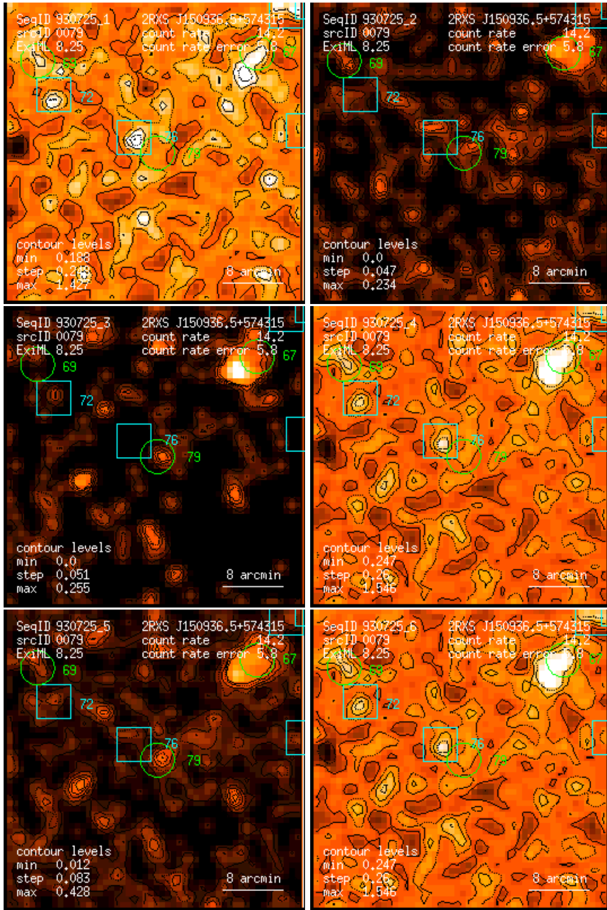
Figure 79: RASS 930725: detection 0079: band rate images, Gaussian filter: (1) PSPC channels 11 – 41, (2) 52 – 90, (3) 91 – 201, (4) 11 – 235, (5) 52 – 201, (6) 11 – 201. Broad band rates in counts/ks. Band rate contour levels in counts/ks/arcmin 2 .
