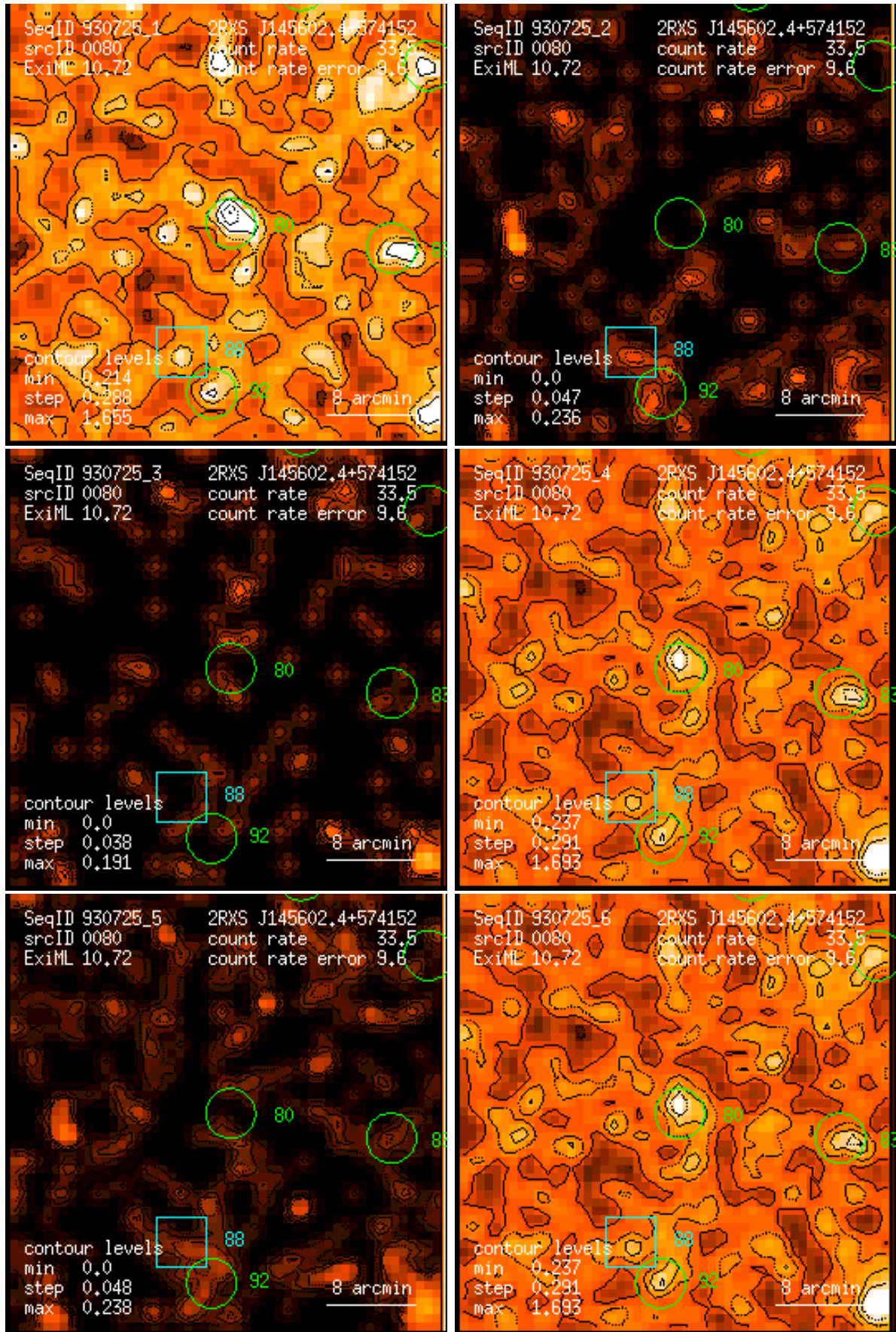
Figure 80: RASS 930725: detection 0080: band rate images, Gaussian filter: (1) PSPC channels 11 – 41, (2) 52 – 90, (3) 91 – 201, (4) 11 – 235, (5) 52 – 201, (6) 11 – 201. Broad band rates in counts/ks. Band rate contour levels in counts/ks/arcmin 2 .
