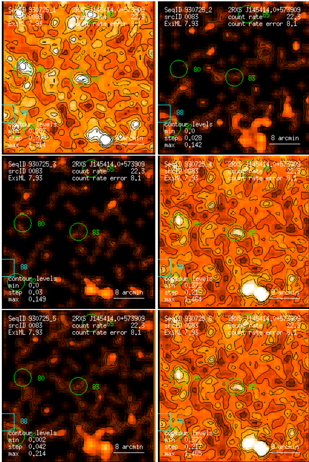
Figure 83: RASS 930725: detection 0083: band rate images, Gaussian filter: (1) PSPC channels 11 – 41, (2) 52 – 90, (3) 91 – 201, (4) 11 – 235, (5) 52 – 201, (6) 11 – 201. Broad band rates in counts/ks. Band rate contour levels in counts/ks/arcmin 2 .
