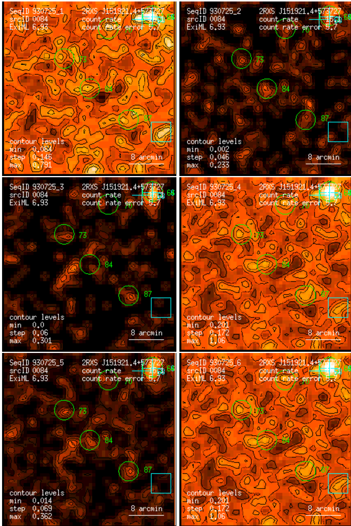
Figure 84: RASS 930725: detection 0084: band rate images, Gaussian filter: (1) PSPC channels 11 – 41, (2) 52 – 90, (3) 91 – 201, (4) 11 – 235, (5) 52 – 201, (6) 11 – 201. Broad band rates in counts/ks. Band rate contour levels in counts/ks/arcmin 2 .
