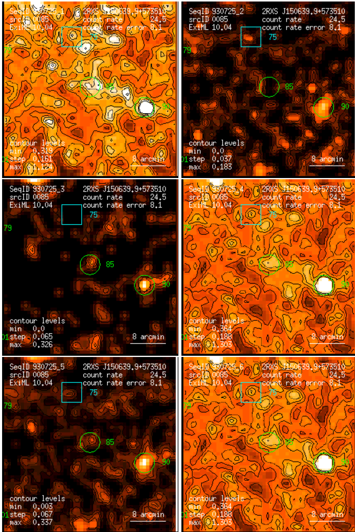
Figure 85: RASS 930725: detection 0085: band rate images, Gaussian filter: (1) PSPC channels 11 – 41, (2) 52 – 90, (3) 91 – 201, (4) 11 – 235, (5) 52 – 201, (6) 11 – 201. Broad band rates in counts/ks. Band rate contour levels in counts/ks/arcmin 2 .
