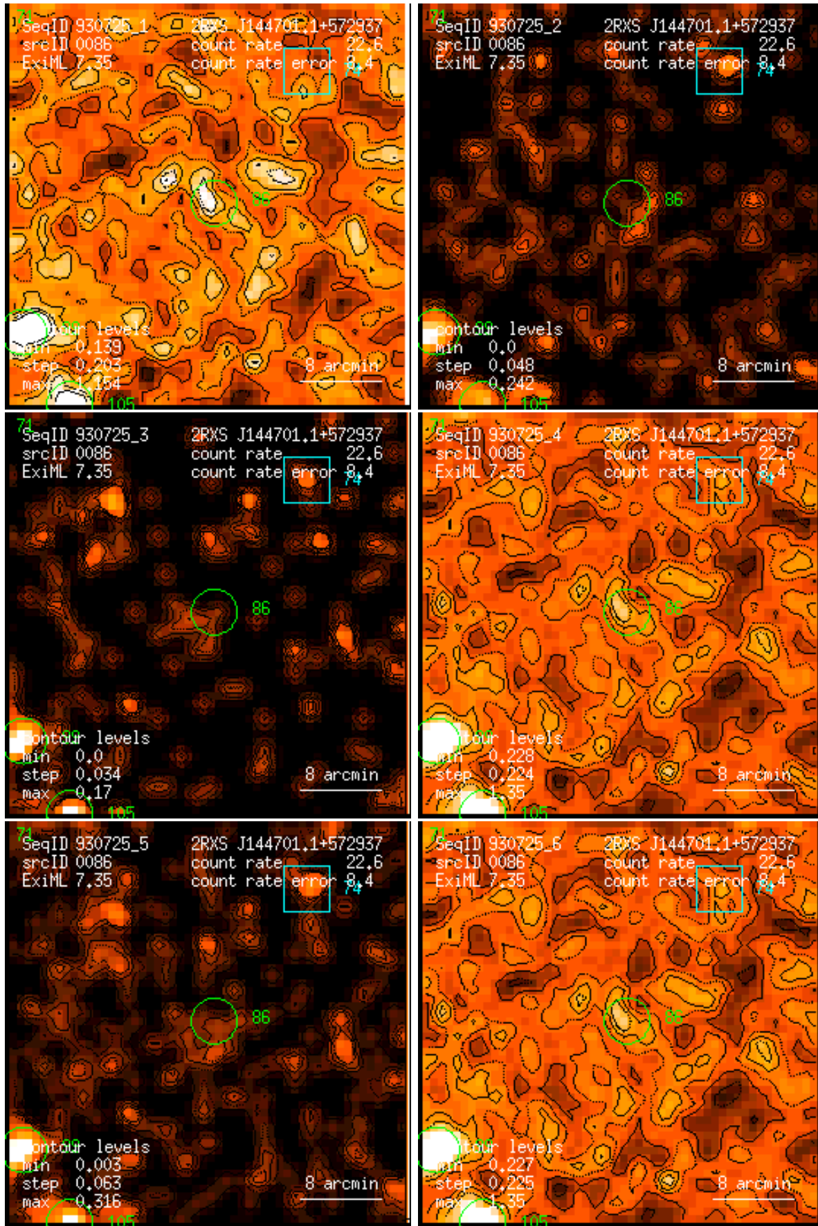
Figure 86: RASS 930725: detection 0086: band rate images, Gaussian filter: (1) PSPC channels 11 – 41, (2) 52 – 90, (3) 91 – 201, (4) 11 – 235, (5) 52 – 201, (6) 11 – 201. Broad band rates in counts/ks. Band rate contour levels in counts/ks/arcmin 2 .
