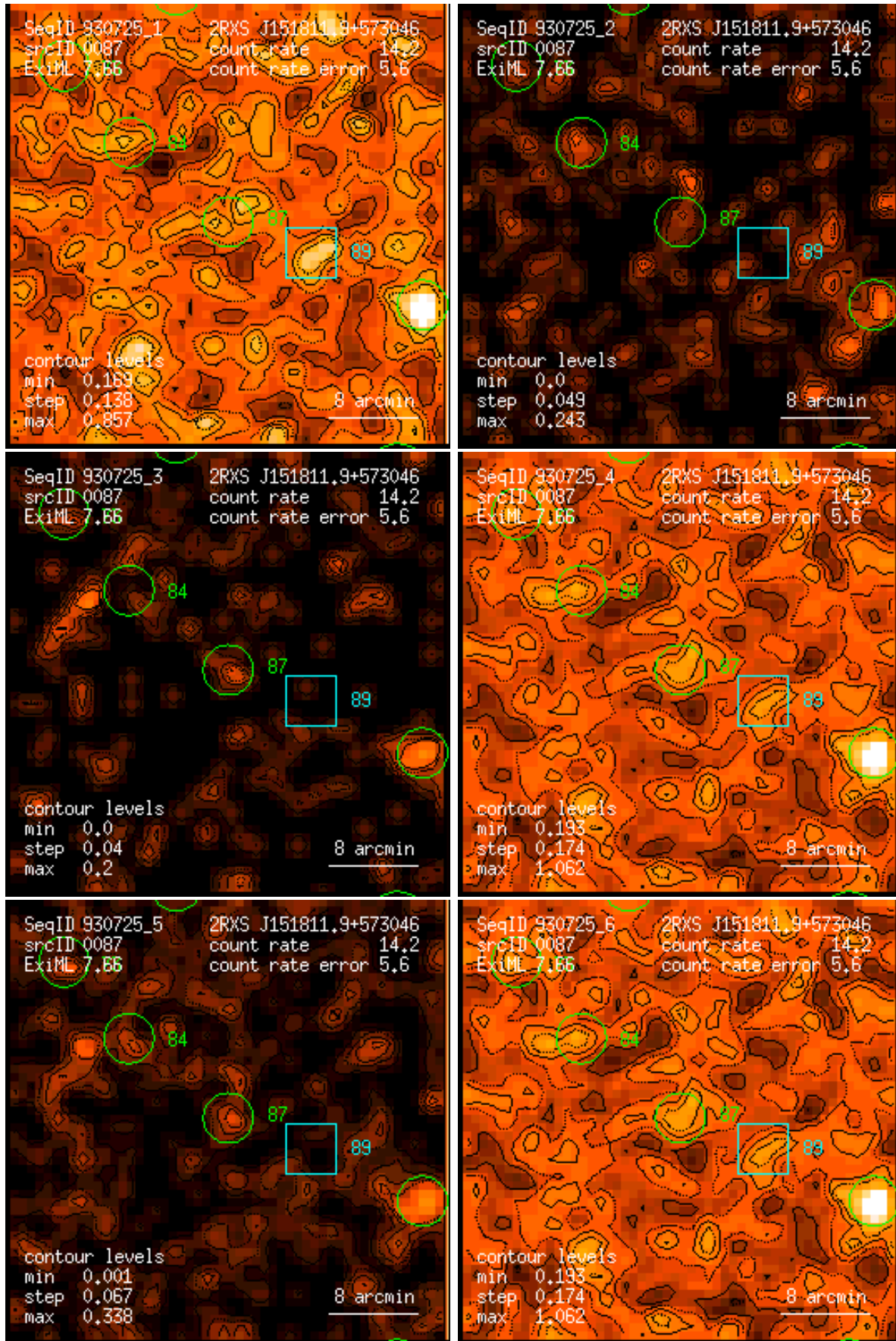
Figure 87: RASS 930725: detection 0087: band rate images, Gaussian filter: (1) PSPC channels 11 – 41, (2) 52 – 90, (3) 91 – 201, (4) 11 – 235, (5) 52 – 201, (6) 11 – 201. Broad band rates in counts/ks. Band rate contour levels in counts/ks/arcmin 2 .
