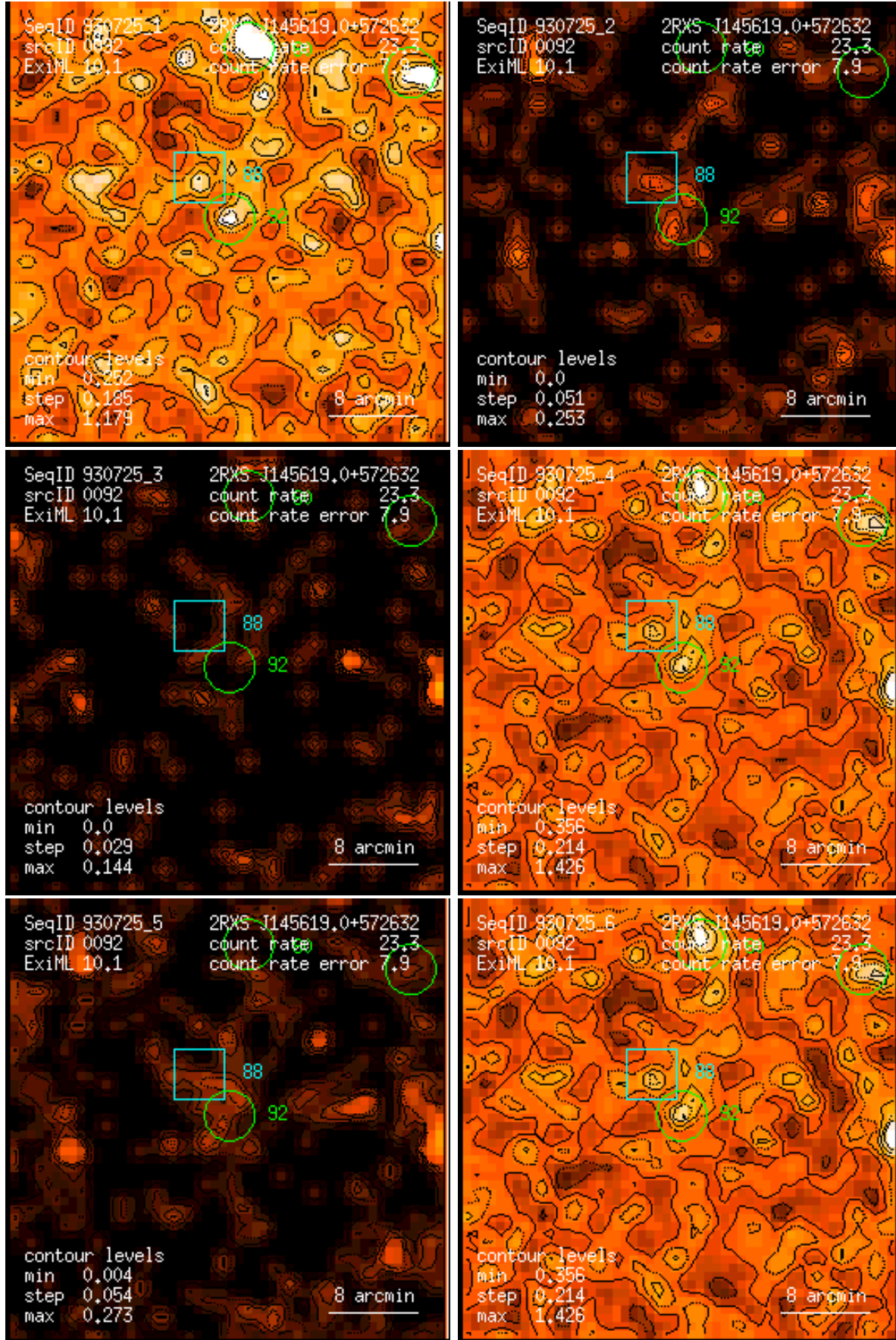
Figure 92: RASS 930725: detection 0092: band rate images, Gaussian filter: (1) PSPC channels 11 – 41, (2) 52 – 90, (3) 91 – 201, (4) 11 – 235, (5) 52 – 201, (6) 11 – 201. Broad band rates in counts/ks. Band rate contour levels in counts/ks/arcmin 2 .
