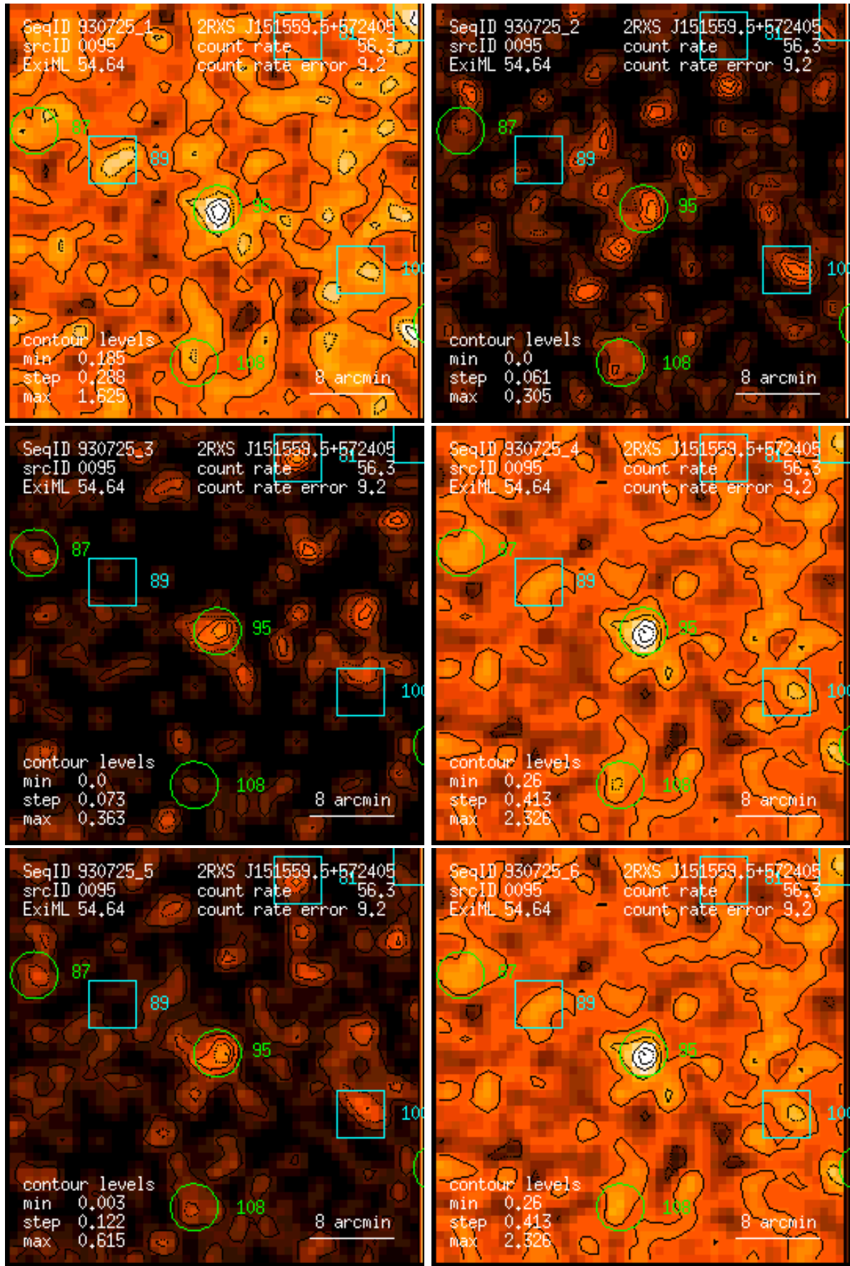
Figure 95: RASS 930725: detection 0095: band rate images, Gaussian filter: (1) PSPC channels 11 – 41, (2) 52 – 90, (3) 91 – 201, (4) 11 – 235, (5) 52 – 201, (6) 11 – 201. Broad band rates in counts/ks. Band rate contour levels in counts/ks/arcmin 2 .
