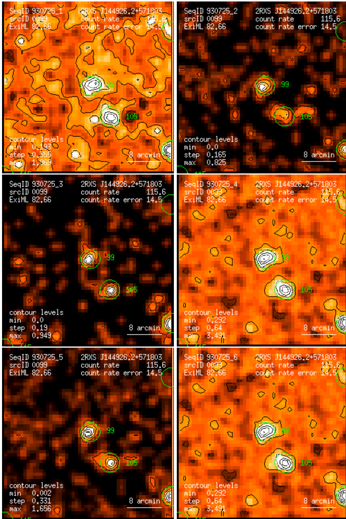
Figure 99: RASS 930725: detection 0099: band rate images, Gaussian filter: (1) PSPC channels 11 – 41, (2) 52 – 90, (3) 91 – 201, (4) 11 – 235, (5) 52 – 201, (6) 11 – 201. Broad band rates in counts/ks. Band rate contour levels in counts/ks/arcmin 2 .
