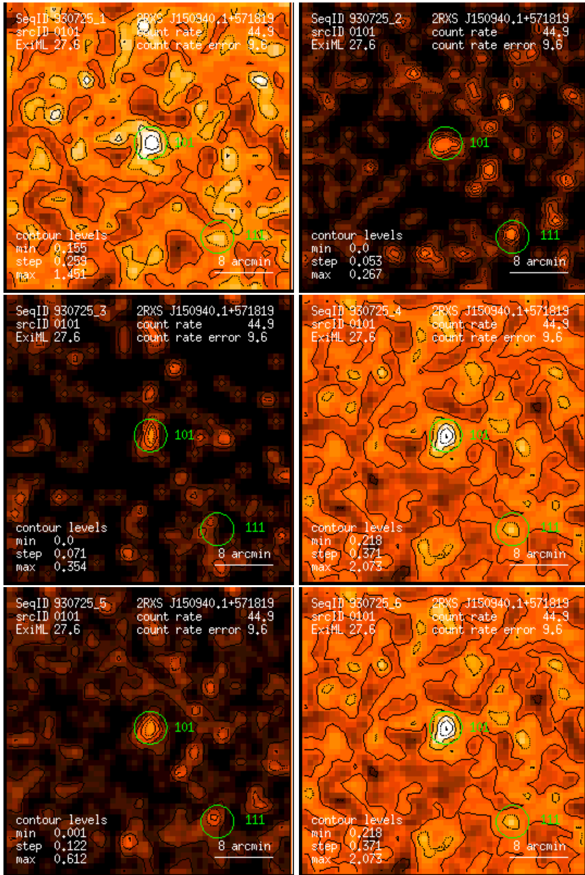
Figure 101: RASS 930725: detection 0101: band rate images, Gaussian filter: (1) PSPC channels 11 – 41, (2) 52 – 90, (3) 91 – 201, (4) 11 – 235, (5) 52 – 201, (6) 11 – 201. Broad band rates in counts/ks. Band rate contour levels in counts/ks/arcmin 2 .
