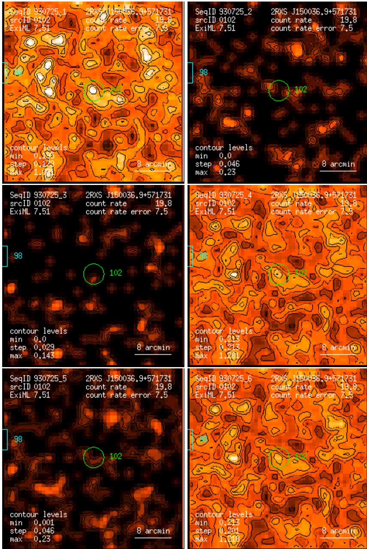
Figure 102: RASS 930725: detection 0102: band rate images, Gaussian filter: (1) PSPC channels 11 – 41, (2) 52 – 90, (3) 91 – 201, (4) 11 – 235, (5) 52 – 201, (6) 11 – 201. Broad band rates in counts/ks. Band rate contour levels in counts/ks/arcmin 2 .
