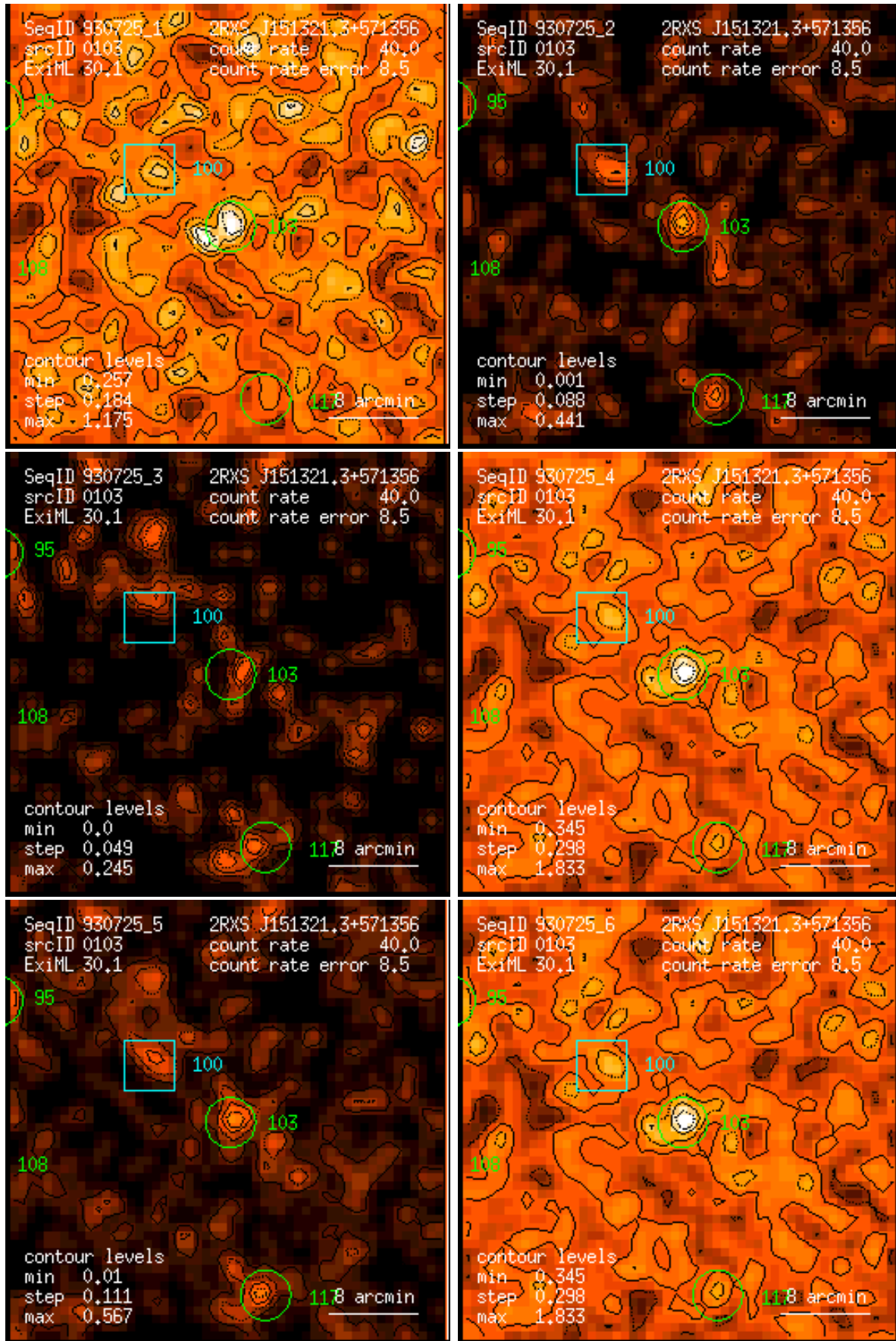
Figure 103: RASS 930725: detection 0103: band rate images, Gaussian filter: (1) PSPC channels 11 – 41, (2) 52 – 90, (3) 91 – 201, (4) 11 – 235, (5) 52 – 201, (6) 11 – 201. Broad band rates in counts/ks. Band rate contour levels in counts/ks/arcmin 2 .
