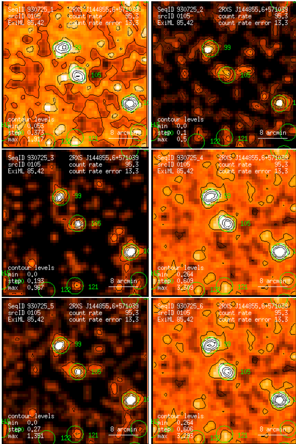
Figure 105: RASS 930725: detection 0105: band rate images, Gaussian filter: (1) PSPC channels 11 – 41, (2) 52 – 90, (3) 91 – 201, (4) 11 – 235, (5) 52 – 201, (6) 11 – 201. Broad band rates in counts/ks. Band rate contour levels in counts/ks/arcmin 2 .
