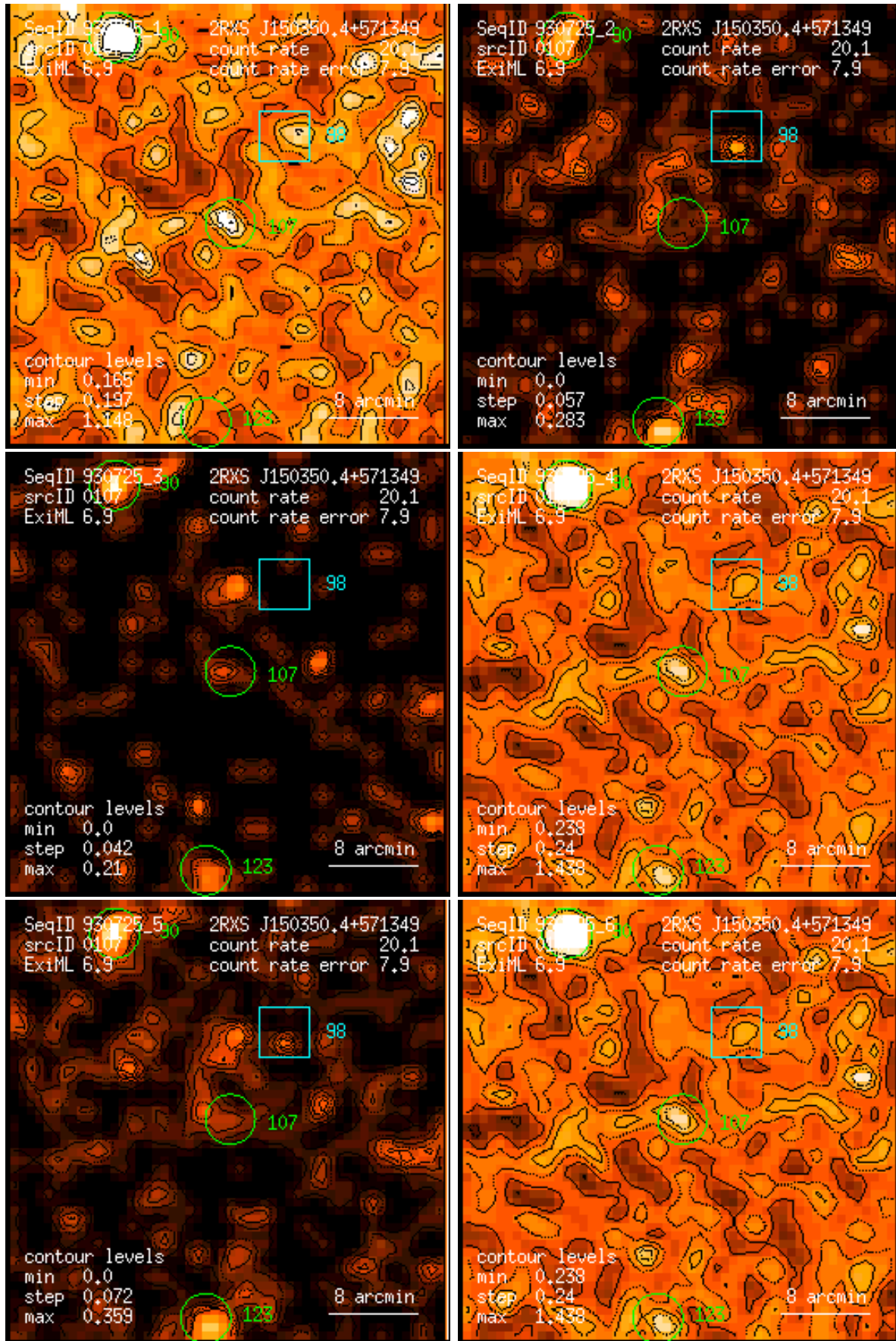
Figure 107: RASS 930725: detection 0107: band rate images, Gaussian filter: (1) PSPC channels 11 – 41, (2) 52 – 90, (3) 91 – 201, (4) 11 – 235, (5) 52 – 201, (6) 11 – 201. Broad band rates in counts/ks. Band rate contour levels in counts/ks/arcmin 2 .
