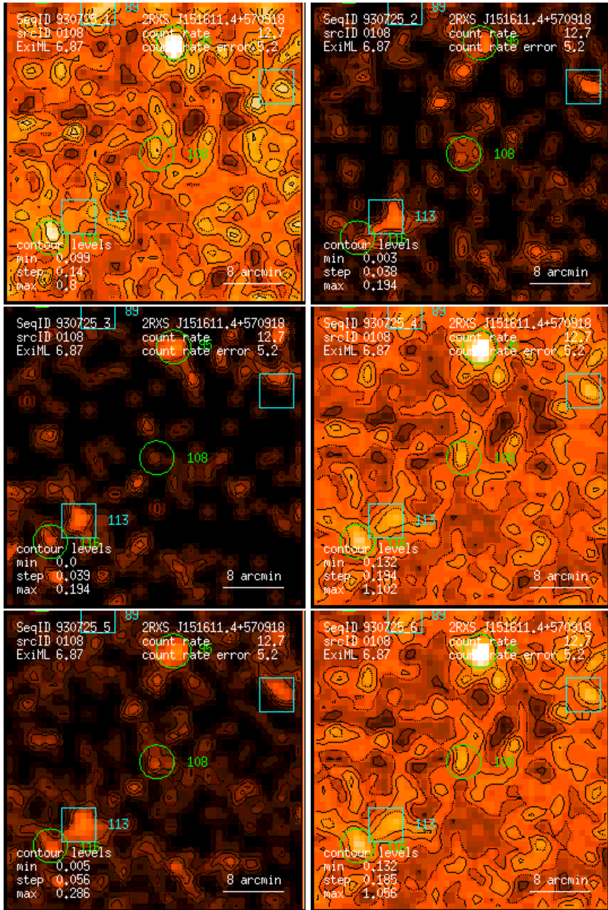
Figure 108: RASS 930725: detection 0108: band rate images, Gaussian filter: (1) PSPC channels 11 – 41, (2) 52 – 90, (3) 91 – 201, (4) 11 – 235, (5) 52 – 201, (6) 11 – 201. Broad band rates in counts/ks. Band rate contour levels in counts/ks/arcmin 2 .
