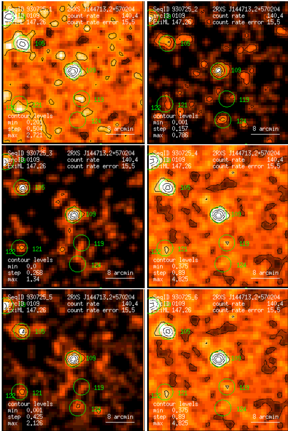
Figure 109: RASS 930725: detection 0109: band rate images, Gaussian filter: (1) PSPC channels 11 – 41, (2) 52 – 90, (3) 91 – 201, (4) 11 – 235, (5) 52 – 201, (6) 11 – 201. Broad band rates in counts/ks. Band rate contour levels in counts/ks/arcmin 2 .
