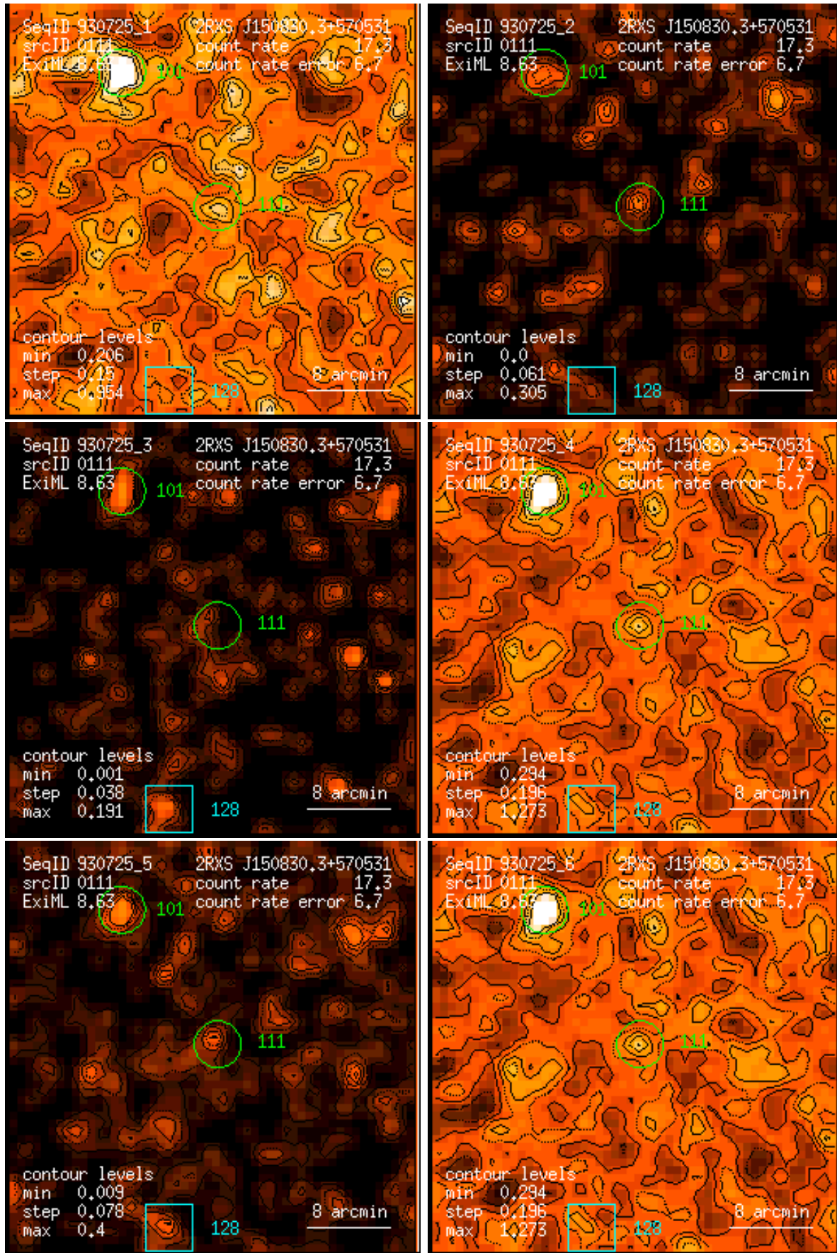
Figure 111: RASS 930725: detection 0111: band rate images, Gaussian filter: (1) PSPC channels 11 – 41, (2) 52 – 90, (3) 91 – 201, (4) 11 – 235, (5) 52 – 201, (6) 11 – 201. Broad band rates in counts/ks. Band rate contour levels in counts/ks/arcmin 2 .
