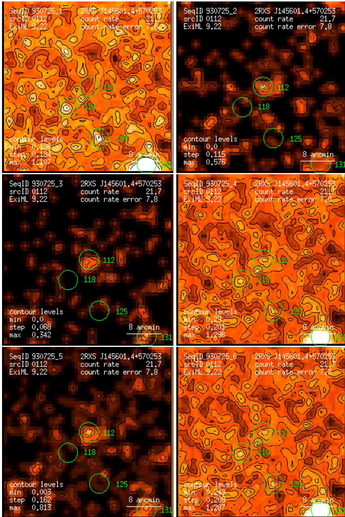
Figure 112: RASS 930725: detection 0112: band rate images, Gaussian filter: (1) PSPC channels 11 – 41, (2) 52 – 90, (3) 91 – 201, (4) 11 – 235, (5) 52 – 201, (6) 11 – 201. Broad band rates in counts/ks. Band rate contour levels in counts/ks/arcmin 2 .
