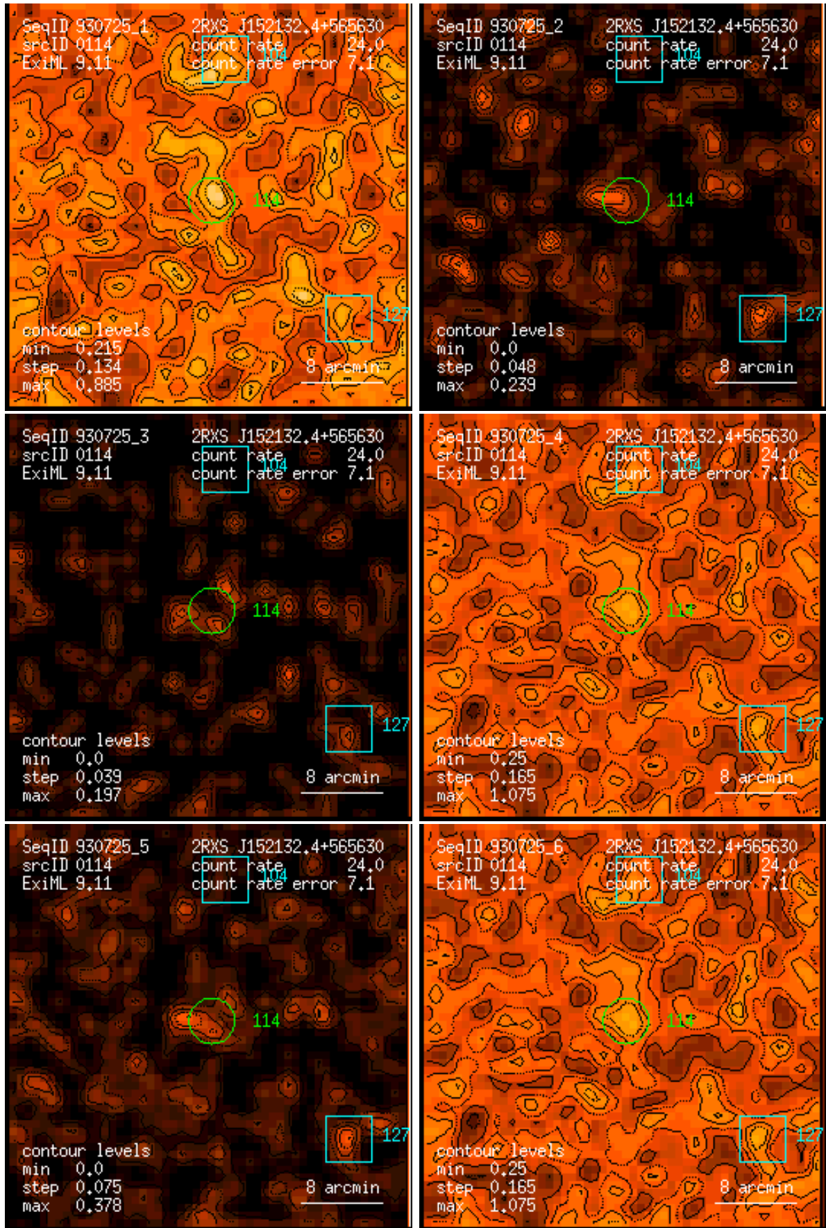
Figure 114: RASS 930725: detection 0114: band rate images, Gaussian filter: (1) PSPC channels 11 – 41, (2) 52 – 90, (3) 91 – 201, (4) 11 – 235, (5) 52 – 201, (6) 11 – 201. Broad band rates in counts/ks. Band rate contour levels in counts/ks/arcmin 2 .
