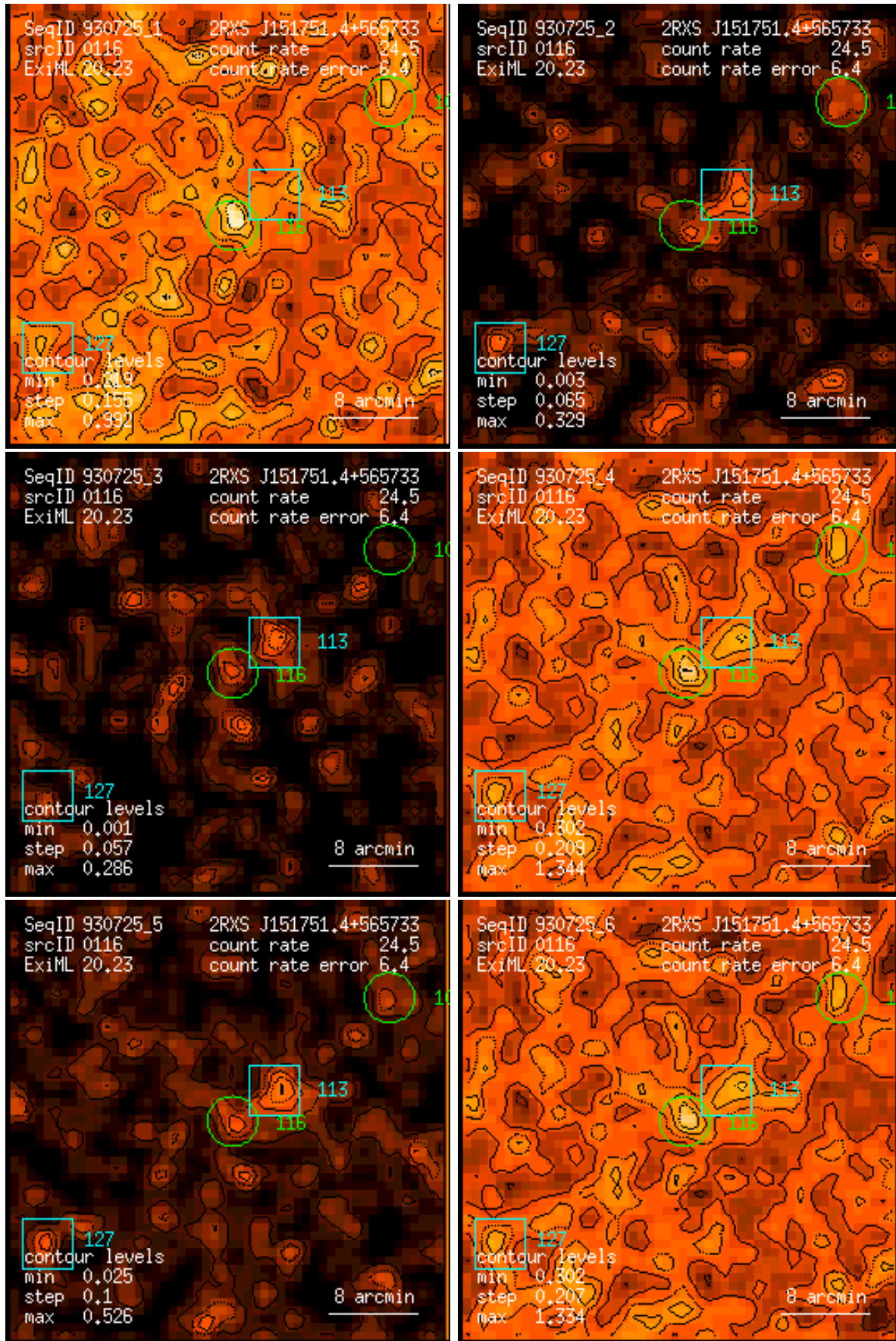
Figure 116: RASS 930725: detection 0116: band rate images, Gaussian filter: (1) PSPC channels 11 – 41, (2) 52 – 90, (3) 91 – 201, (4) 11 – 235, (5) 52 – 201, (6) 11 – 201. Broad band rates in counts/ks. Band rate contour levels in counts/ks/arcmin 2 .
