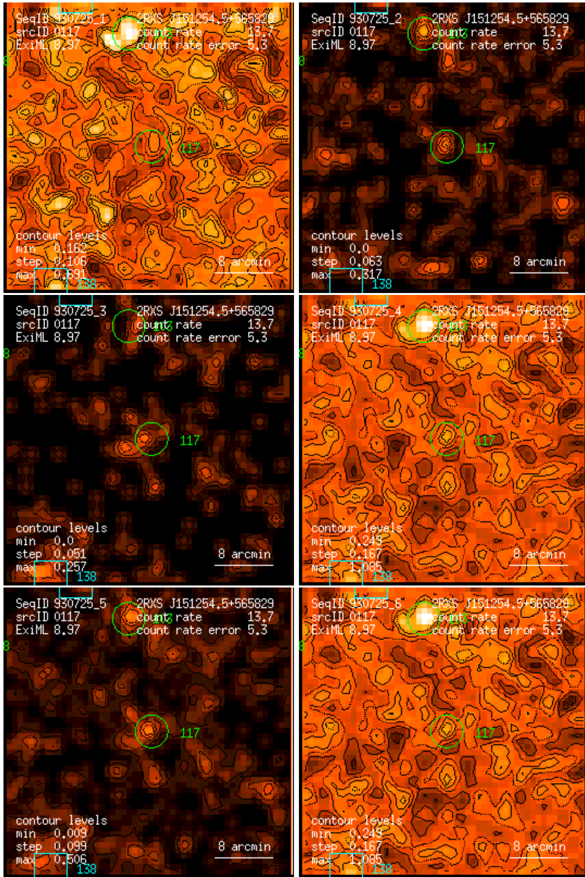
Figure 117: RASS 930725: detection 0117: band rate images, Gaussian filter: (1) PSPC channels 11 – 41, (2) 52 – 90, (3) 91 – 201, (4) 11 – 235, (5) 52 – 201, (6) 11 – 201. Broad band rates in counts/ks. Band rate contour levels in counts/ks/arcmin 2 .
