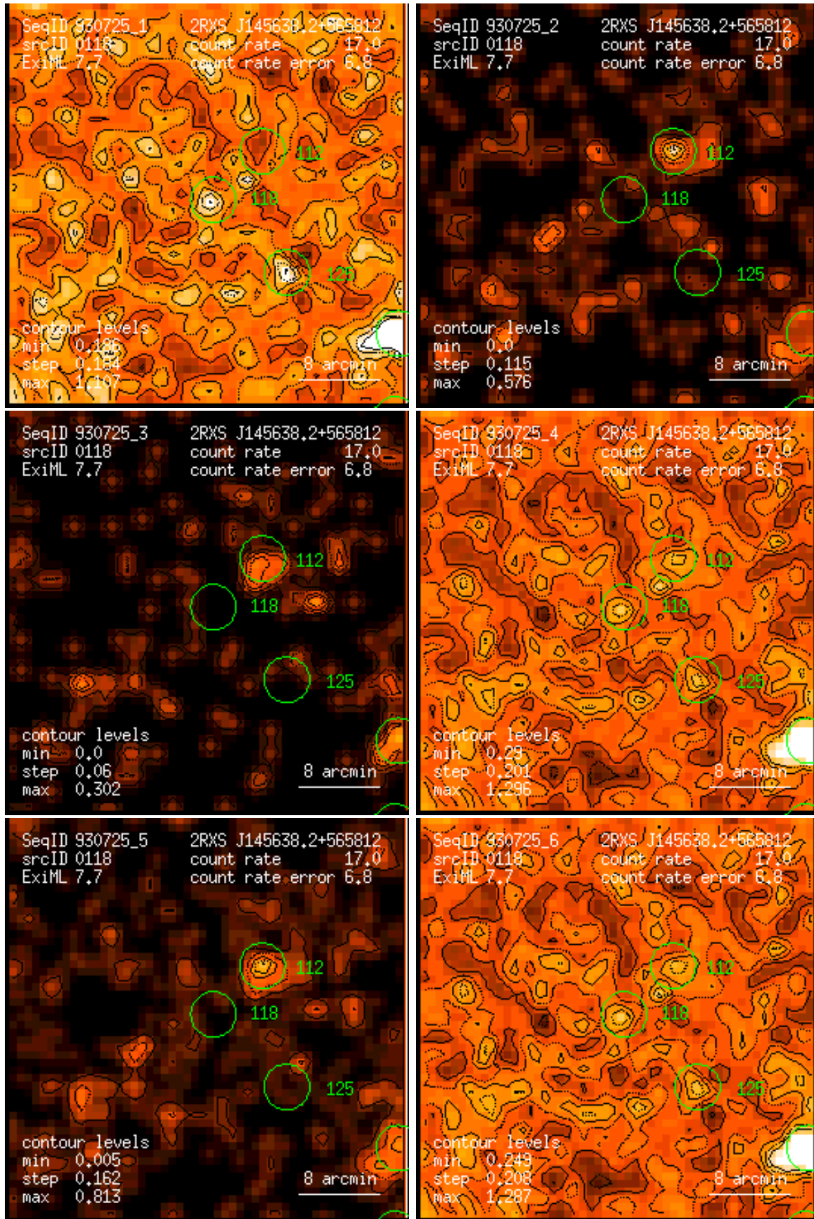
Figure 118: RASS 930725: detection 0118: band rate images, Gaussian filter: (1) PSPC channels 11 – 41, (2) 52 – 90, (3) 91 – 201, (4) 11 – 235, (5) 52 – 201, (6) 11 – 201. Broad band rates in counts/ks. Band rate contour levels in counts/ks/arcmin 2 .
