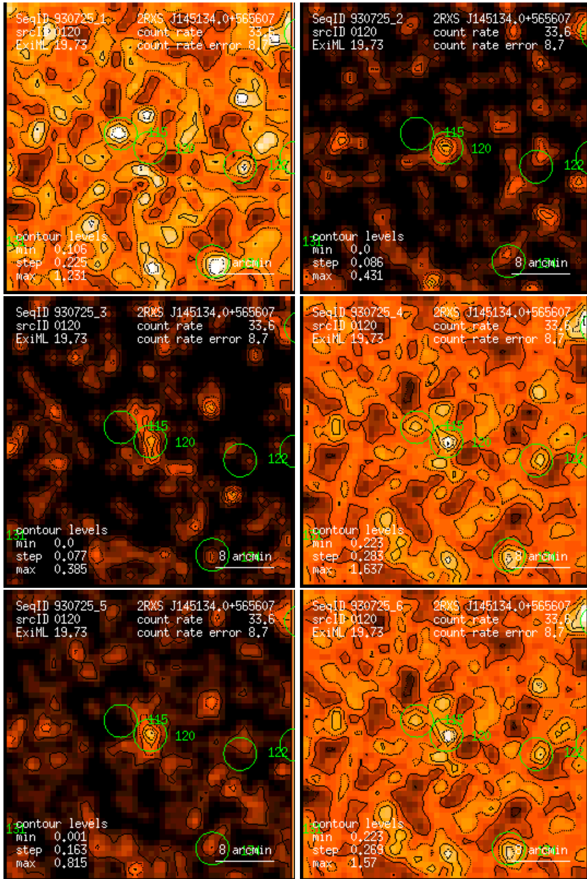
Figure 120: RASS 930725: detection 0120: band rate images, Gaussian filter: (1) PSPC channels 11 – 41, (2) 52 – 90, (3) 91 – 201, (4) 11 – 235, (5) 52 – 201, (6) 11 – 201. Broad band rates in counts/ks. Band rate contour levels in counts/ks/arcmin 2 .
