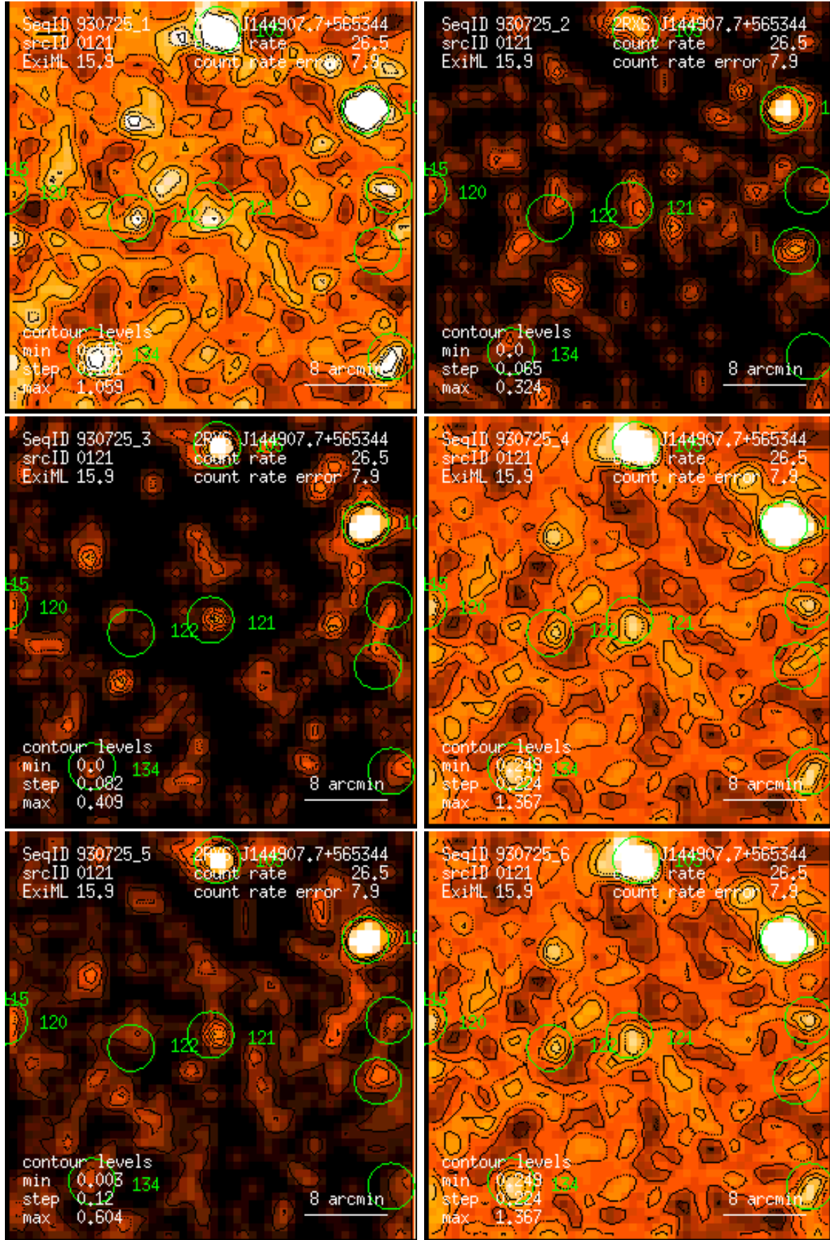
Figure 121: RASS 930725: detection 0121: band rate images, Gaussian filter: (1) PSPC channels 11 – 41, (2) 52 – 90, (3) 91 – 201, (4) 11 – 235, (5) 52 – 201, (6) 11 – 201. Broad band rates in counts/ks. Band rate contour levels in counts/ks/arcmin 2 .
