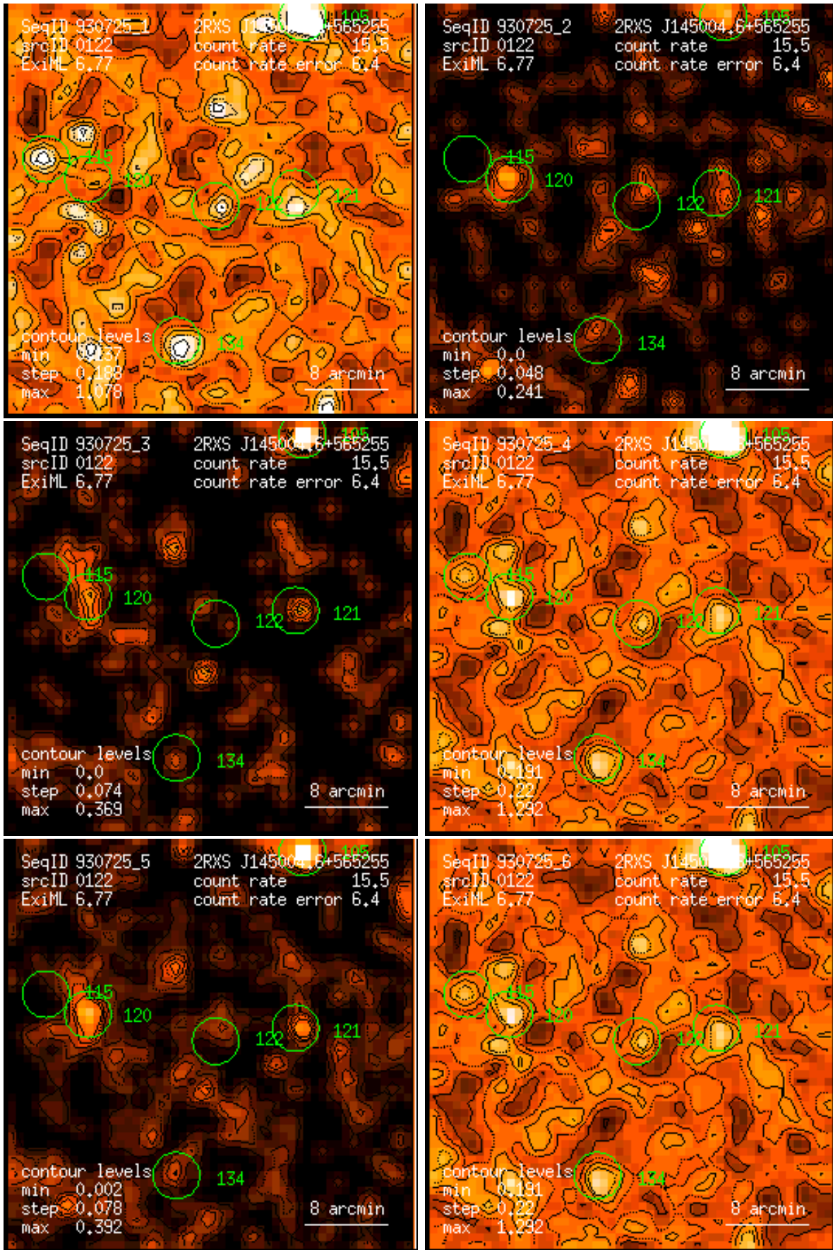
Figure 122: RASS 930725: detection 0122: band rate images, Gaussian filter: (1) PSPC channels 11 – 41, (2) 52 – 90, (3) 91 – 201, (4) 11 – 235, (5) 52 – 201, (6) 11 – 201. Broad band rates in counts/ks. Band rate contour levels in counts/ks/arcmin 2 .
