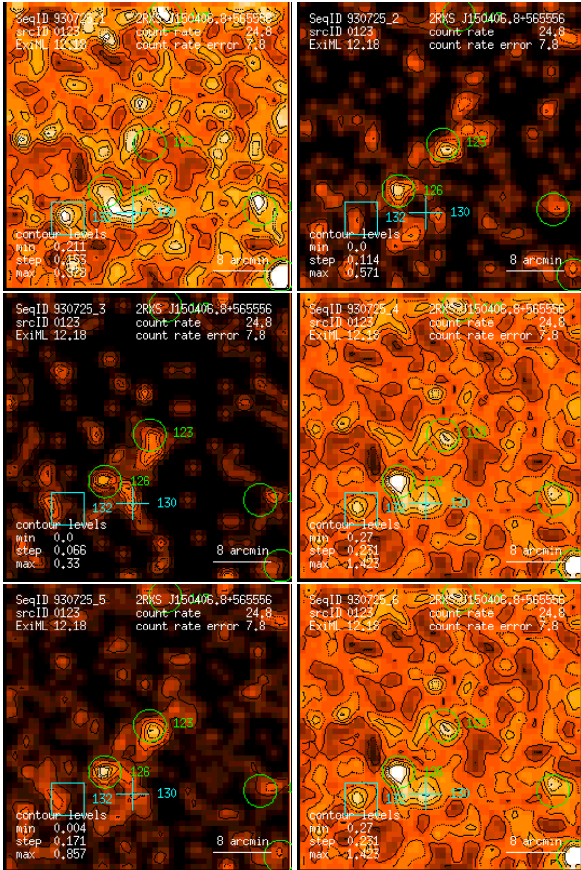
Figure 123: RASS 930725: detection 0123: band rate images, Gaussian filter: (1) PSPC channels 11 – 41, (2) 52 – 90, (3) 91 – 201, (4) 11 – 235, (5) 52 – 201, (6) 11 – 201. Broad band rates in counts/ks. Band rate contour levels in counts/ks/arcmin 2 .
