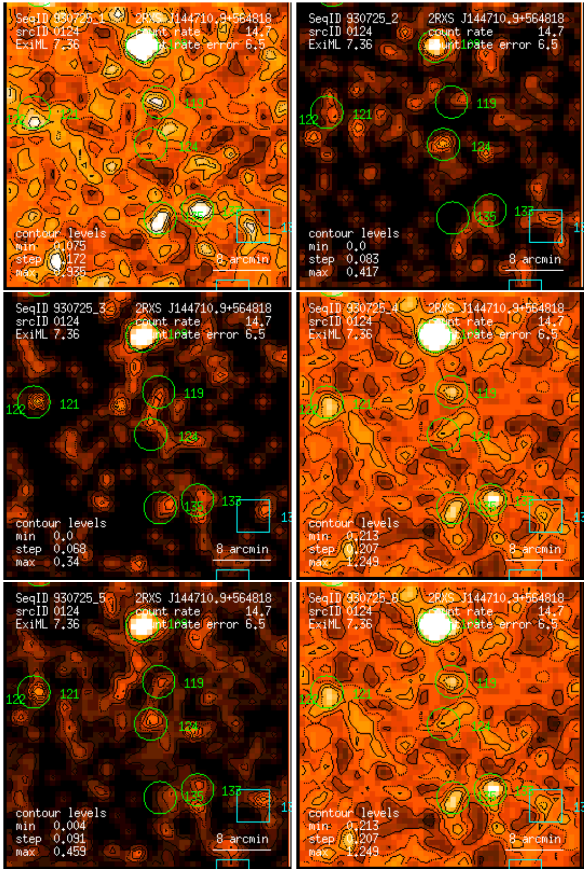
Figure 124: RASS 930725: detection 0124: band rate images, Gaussian filter: (1) PSPC channels 11 – 41, (2) 52 – 90, (3) 91 – 201, (4) 11 – 235, (5) 52 – 201, (6) 11 – 201. Broad band rates in counts/ks. Band rate contour levels in counts/ks/arcmin 2 .
