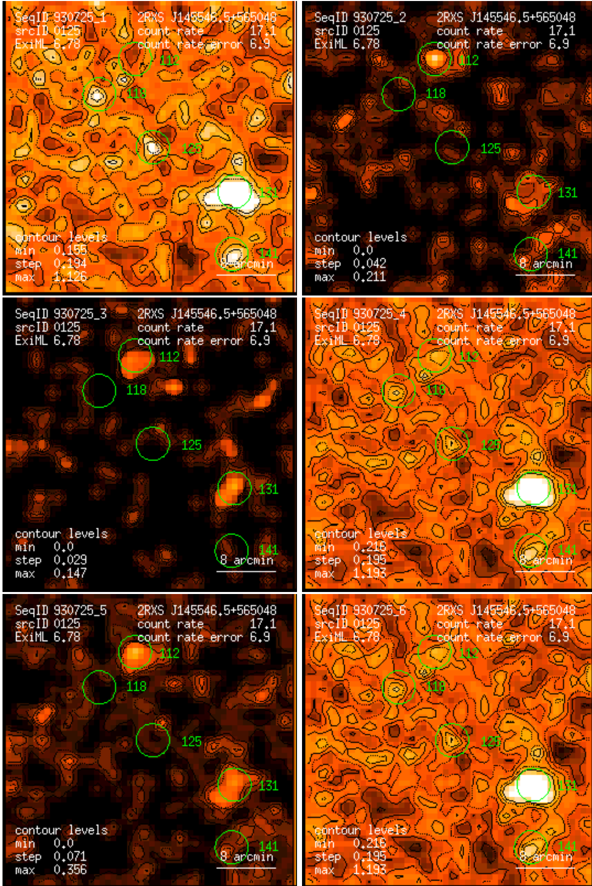
Figure 125: RASS 930725: detection 0125: band rate images, Gaussian filter: (1) PSPC channels 11 – 41, (2) 52 – 90, (3) 91 – 201, (4) 11 – 235, (5) 52 – 201, (6) 11 – 201. Broad band rates in counts/ks. Band rate contour levels in counts/ks/arcmin 2 .
