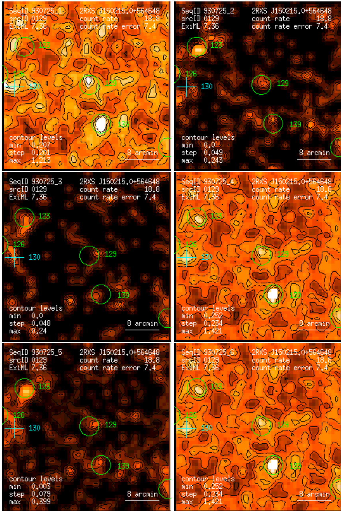
Figure 129: RASS 930725: detection 0129: band rate images, Gaussian filter: (1) PSPC channels 11 – 41, (2) 52 – 90, (3) 91 – 201, (4) 11 – 235, (5) 52 – 201, (6) 11 – 201. Broad band rates in counts/ks. Band rate contour levels in counts/ks/arcmin 2 .
