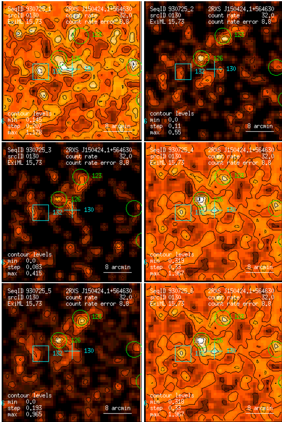
Figure 130: RASS 930725: detection 0130: band rate images, Gaussian filter: (1) PSPC channels 11 – 41, (2) 52 – 90, (3) 91 – 201, (4) 11 – 235, (5) 52 – 201, (6) 11 – 201. Broad band rates in counts/ks. Band rate contour levels in counts/ks/arcmin 2 .
