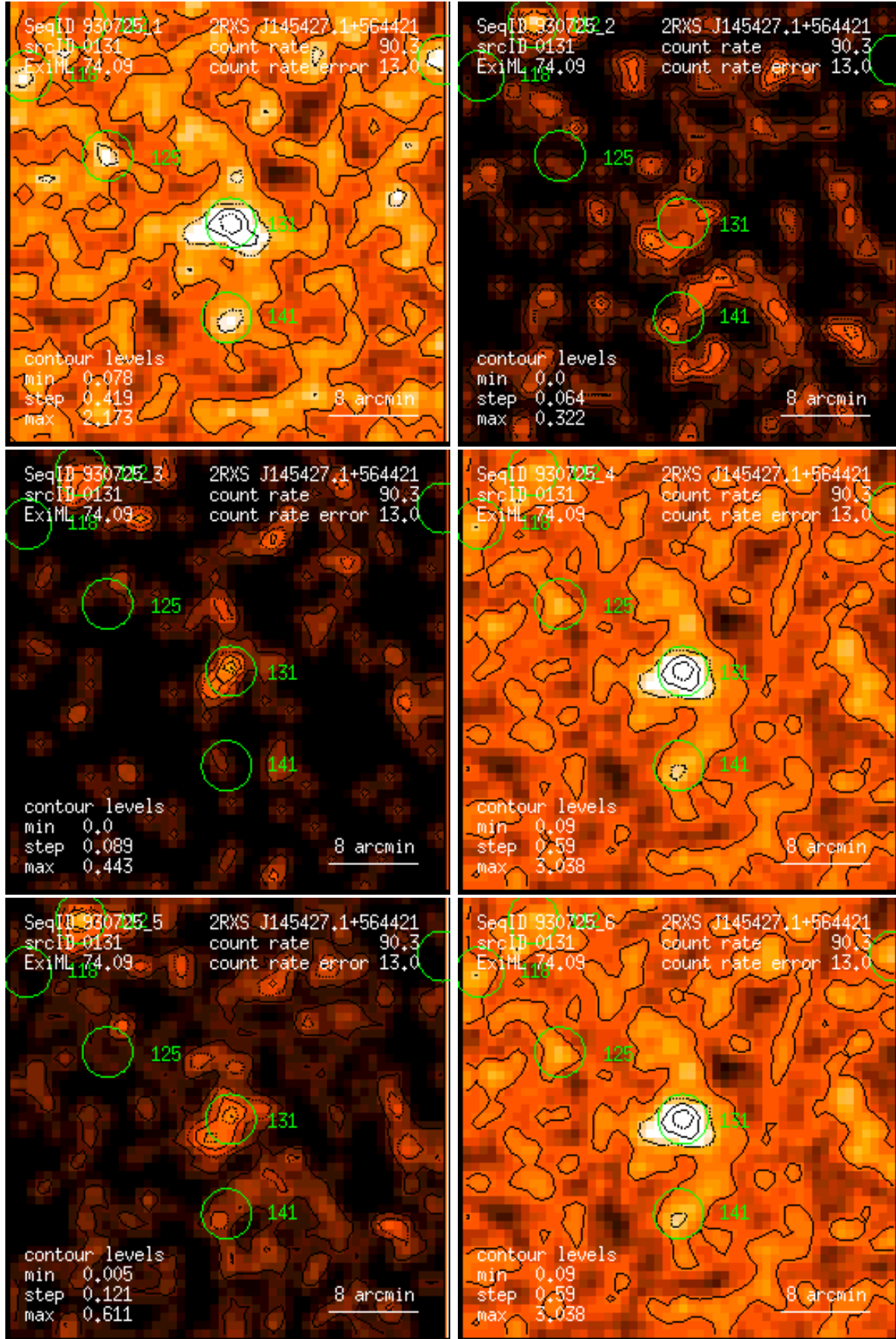
Figure 131: RASS 930725: detection 0131: band rate images, Gaussian filter: (1) PSPC channels 11 – 41, (2) 52 – 90, (3) 91 – 201, (4) 11 – 235, (5) 52 – 201, (6) 11 – 201. Broad band rates in counts/ks. Band rate contour levels in counts/ks/arcmin 2 .
