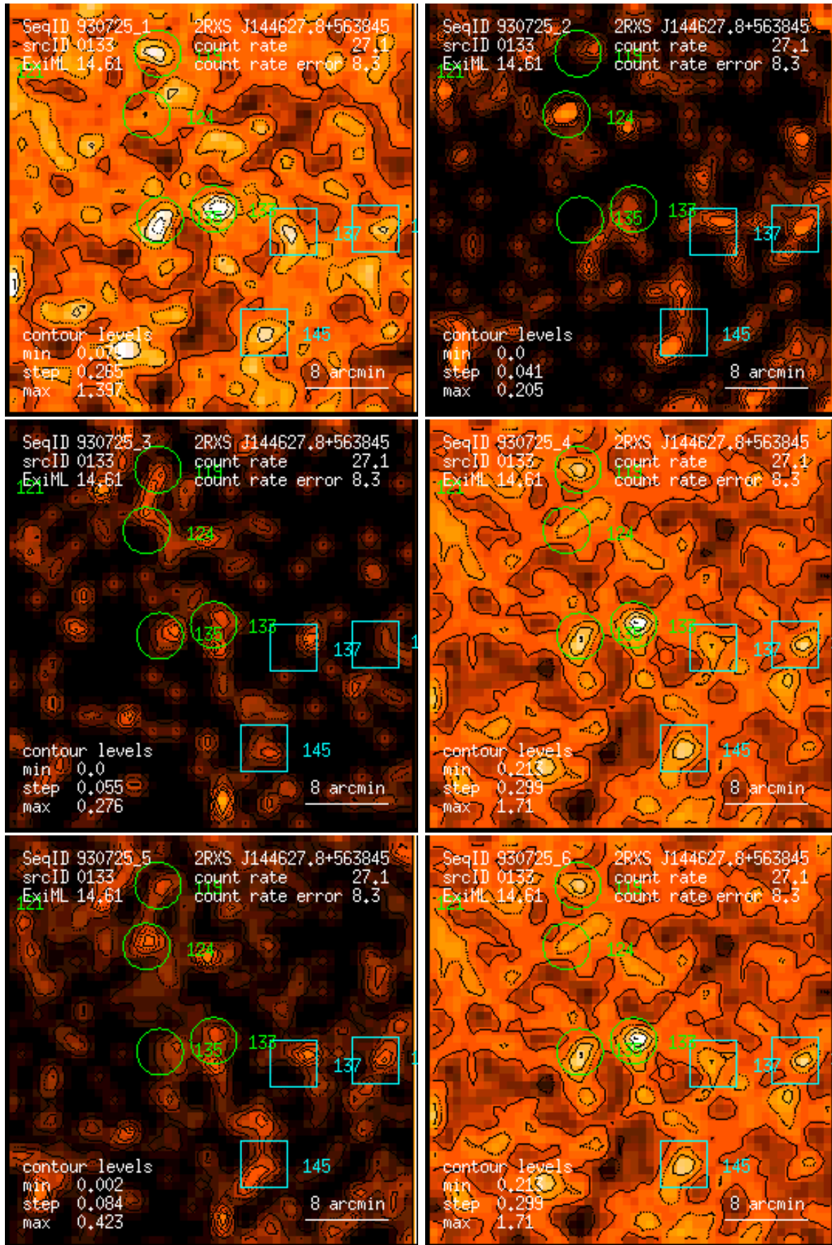
Figure 133: RASS 930725: detection 0133: band rate images, Gaussian filter: (1) PSPC channels 11 – 41, (2) 52 – 90, (3) 91 – 201, (4) 11 – 235, (5) 52 – 201, (6) 11 – 201. Broad band rates in counts/ks. Band rate contour levels in counts/ks/arcmin 2 .
