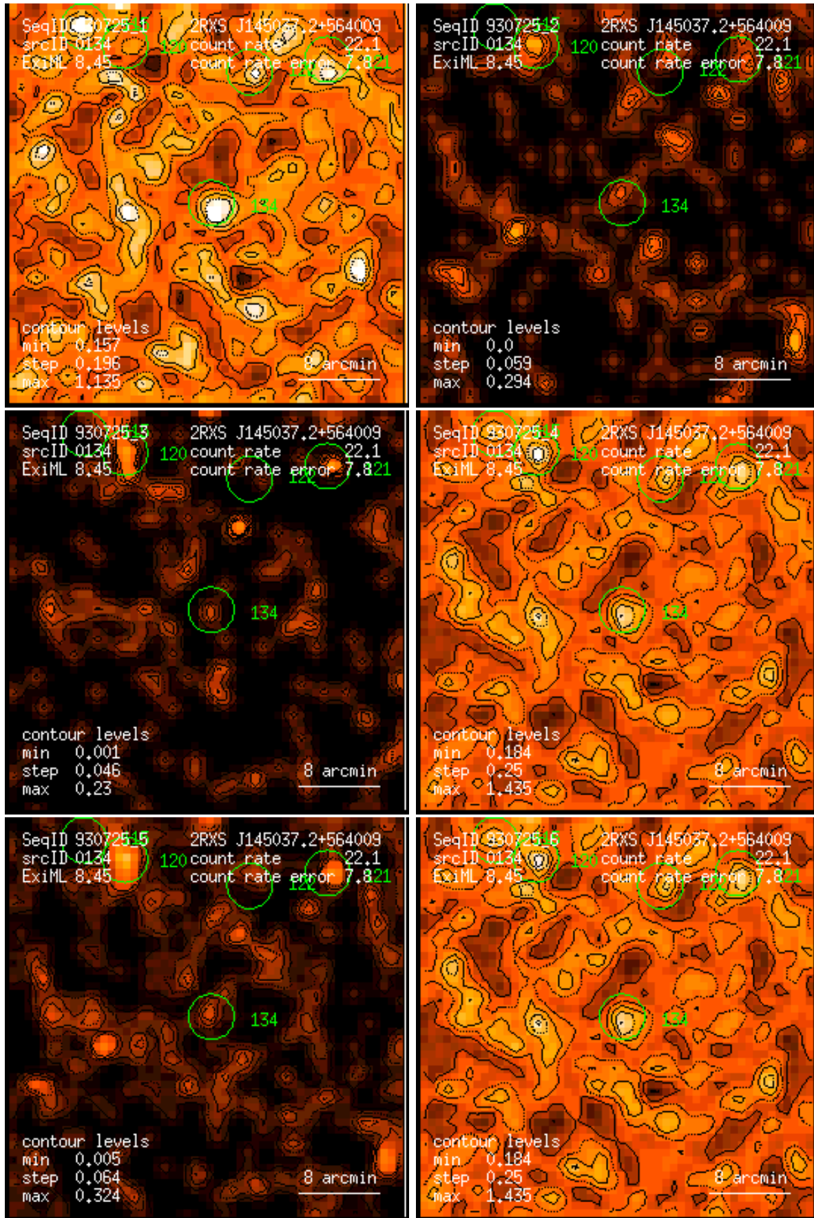
Figure 134: RASS 930725: detection 0134: band rate images, Gaussian filter: (1) PSPC channels 11 – 41, (2) 52 – 90, (3) 91 – 201, (4) 11 – 235, (5) 52 – 201, (6) 11 – 201. Broad band rates in counts/ks. Band rate contour levels in counts/ks/arcmin 2 .
