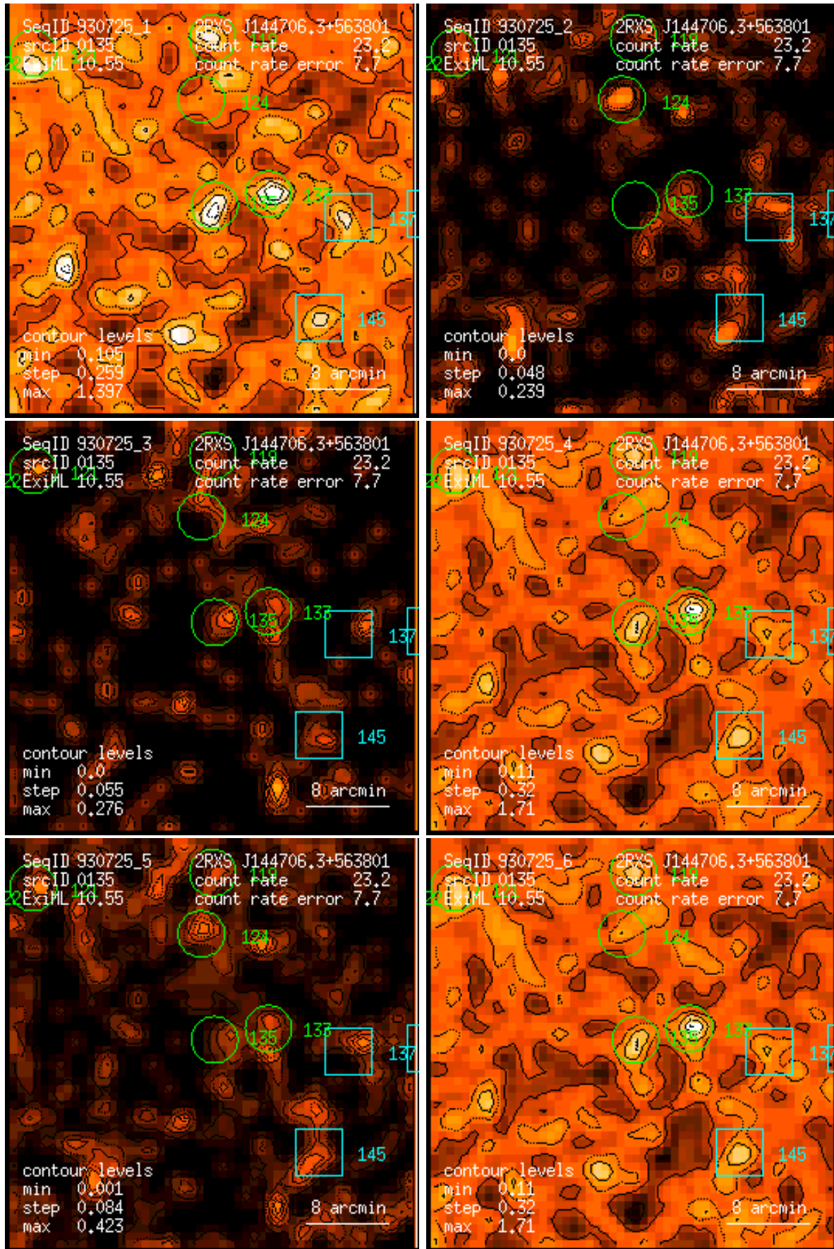
Figure 135: RASS 930725: detection 0135: band rate images, Gaussian filter: (1) PSPC channels 11 – 41, (2) 52 – 90, (3) 91 – 201, (4) 11 – 235, (5) 52 – 201, (6) 11 – 201. Broad band rates in counts/ks. Band rate contour levels in counts/ks/arcmin 2 .
