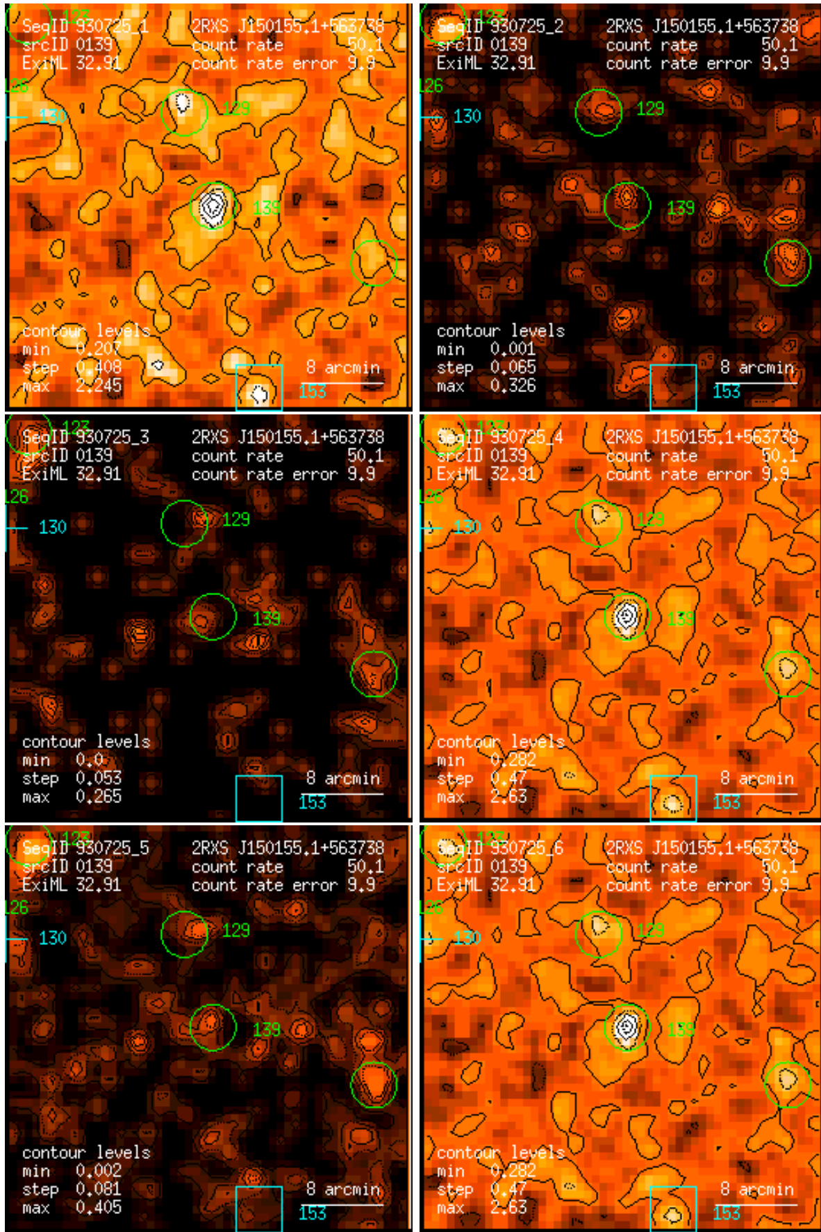
Figure 139: RASS 930725: detection 0139: band rate images, Gaussian filter: (1) PSPC channels 11 – 41, (2) 52 – 90, (3) 91 – 201, (4) 11 – 235, (5) 52 – 201, (6) 11 – 201. Broad band rates in counts/ks. Band rate contour levels in counts/ks/arcmin 2 .
