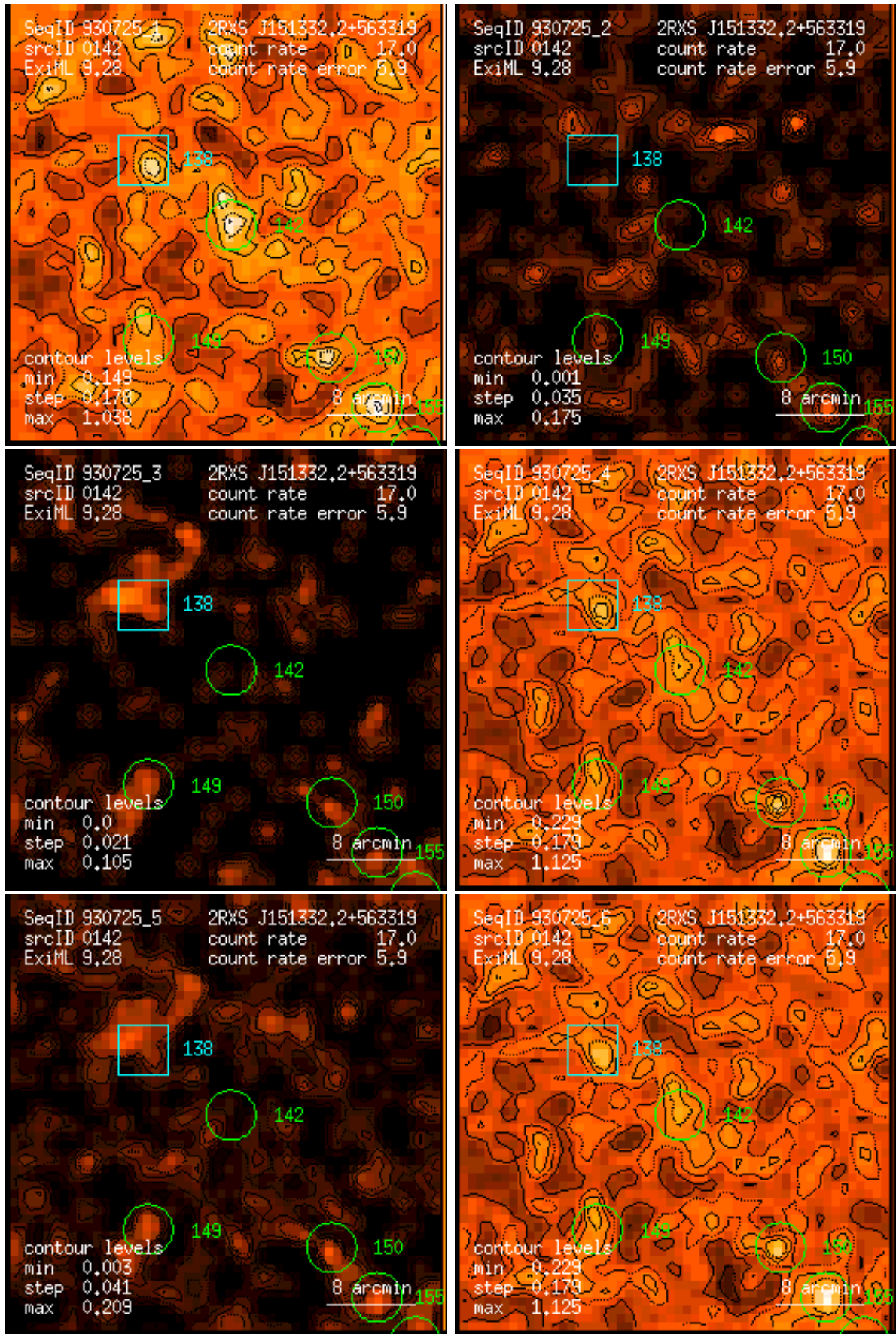
Figure 142: RASS 930725: detection 0142: band rate images, Gaussian filter: (1) PSPC channels 11 – 41, (2) 52 – 90, (3) 91 – 201, (4) 11 – 235, (5) 52 – 201, (6) 11 – 201. Broad band rates in counts/ks. Band rate contour levels in counts/ks/arcmin 2 .
