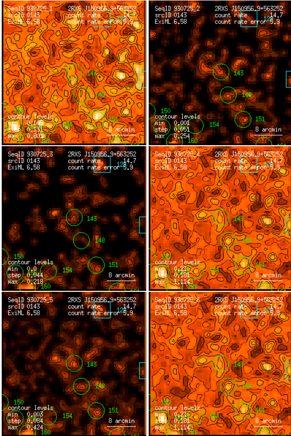
Figure 143: RASS 930725: detection 0143: band rate images, Gaussian filter: (1) PSPC channels 11 – 41, (2) 52 – 90, (3) 91 – 201, (4) 11 – 235, (5) 52 – 201, (6) 11 – 201. Broad band rates in counts/ks. Band rate contour levels in counts/ks/arcmin 2 .
