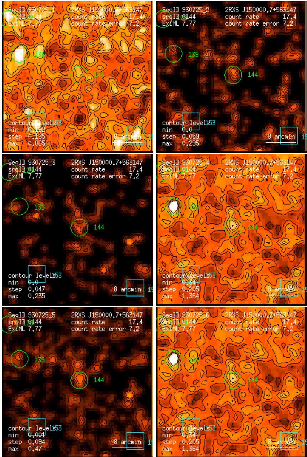
Figure 144: RASS 930725: detection 0144: band rate images, Gaussian filter: (1) PSPC channels 11 – 41, (2) 52 – 90, (3) 91 – 201, (4) 11 – 235, (5) 52 – 201, (6) 11 – 201. Broad band rates in counts/ks. Band rate contour levels in counts/ks/arcmin 2 .
