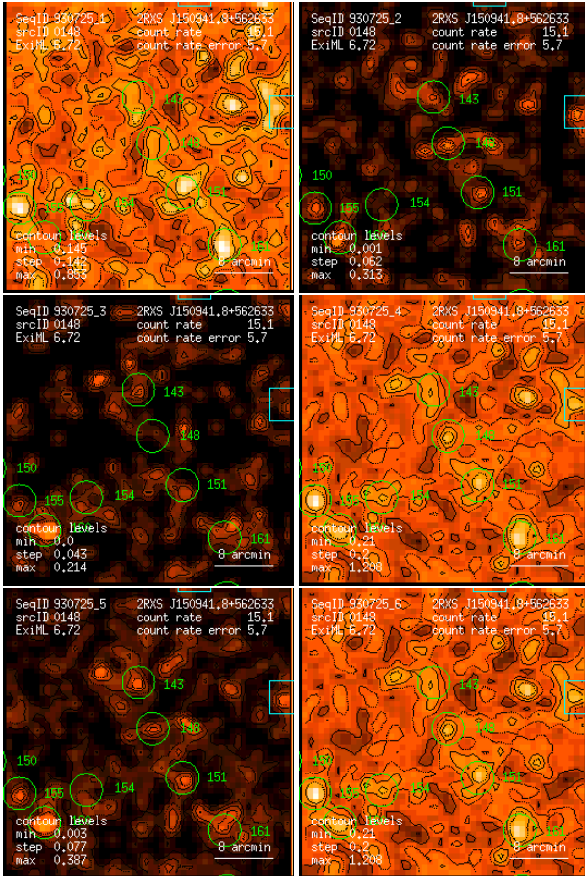
Figure 148: RASS 930725: detection 0148: band rate images, Gaussian filter: (1) PSPC channels 11 – 41, (2) 52 – 90, (3) 91 – 201, (4) 11 – 235, (5) 52 – 201, (6) 11 – 201. Broad band rates in counts/ks. Band rate contour levels in counts/ks/arcmin 2 .
