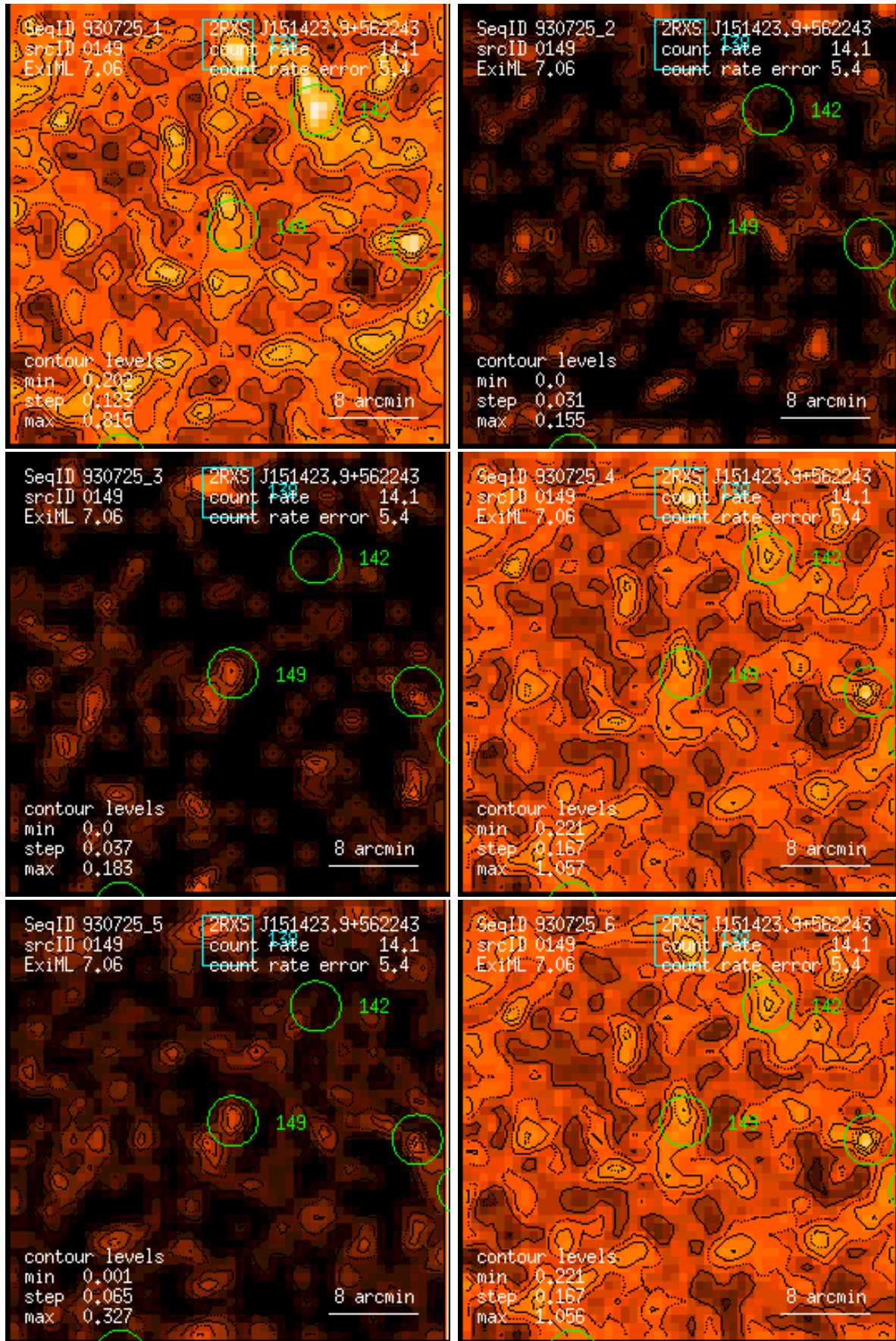
Figure 149: RASS 930725: detection 0149: band rate images, Gaussian filter: (1) PSPC channels 11 – 41, (2) 52 – 90, (3) 91 – 201, (4) 11 – 235, (5) 52 – 201, (6) 11 – 201. Broad band rates in counts/ks. Band rate contour levels in counts/ks/arcmin 2 .
