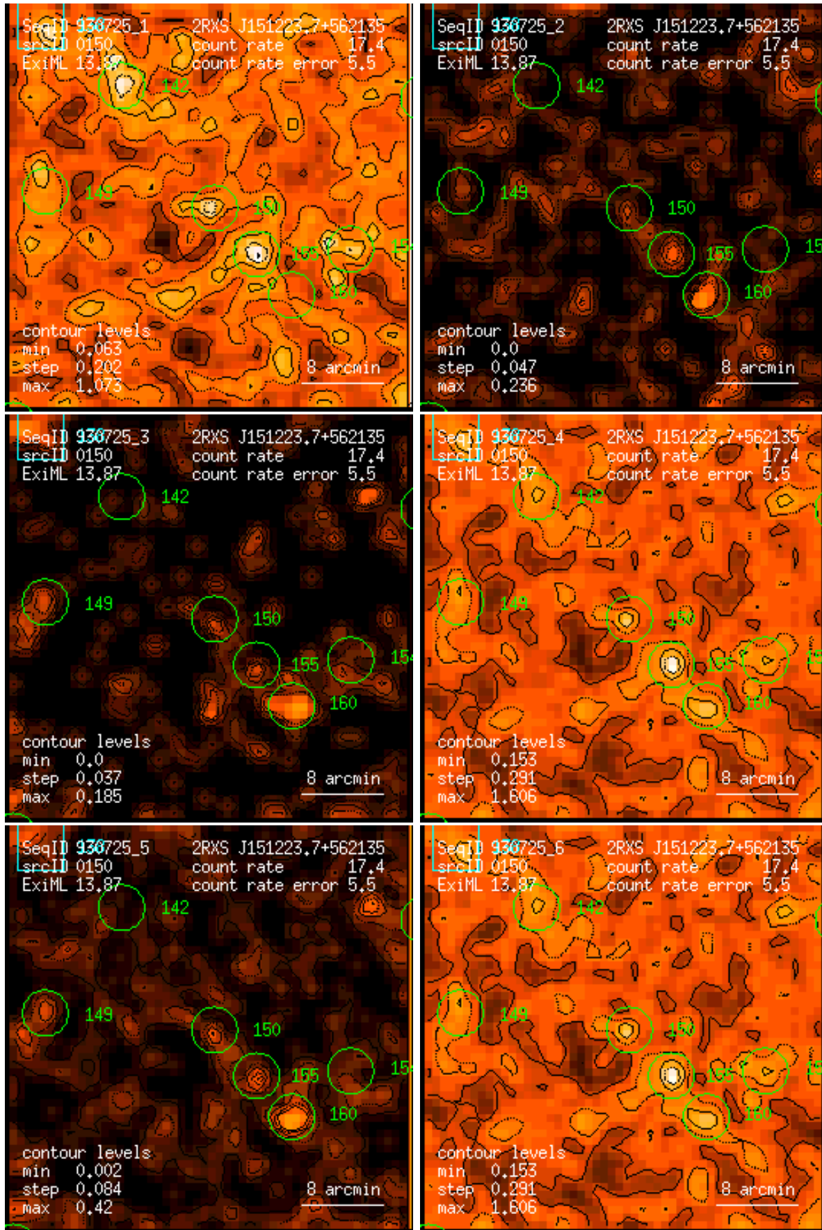
Figure 150: RASS 930725: detection 0150: band rate images, Gaussian filter: (1) PSPC channels 11 – 41, (2) 52 – 90, (3) 91 – 201, (4) 11 – 235, (5) 52 – 201, (6) 11 – 201. Broad band rates in counts/ks. Band rate contour levels in counts/ks/arcmin 2 .
